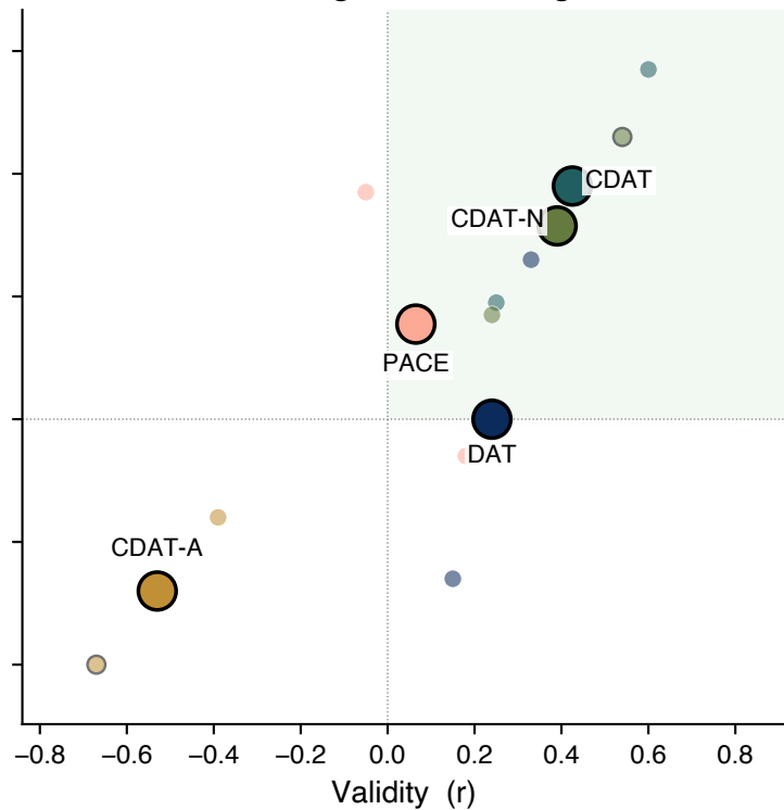
Divergent Thinking
