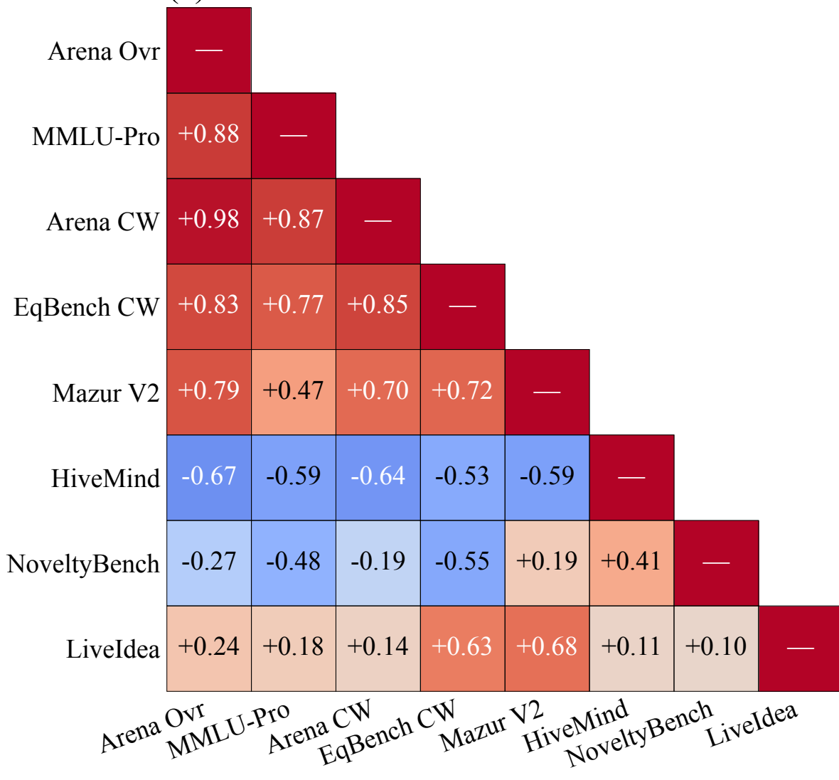
(a) Inter-benchmark correlations
