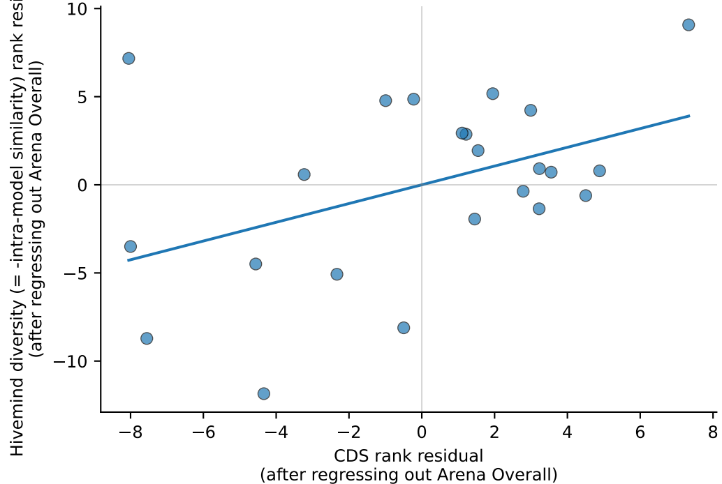
CDS vs Hivemind diversity (= -intra-model similarity) partial Spearman \rho = +0.337 , n=23
