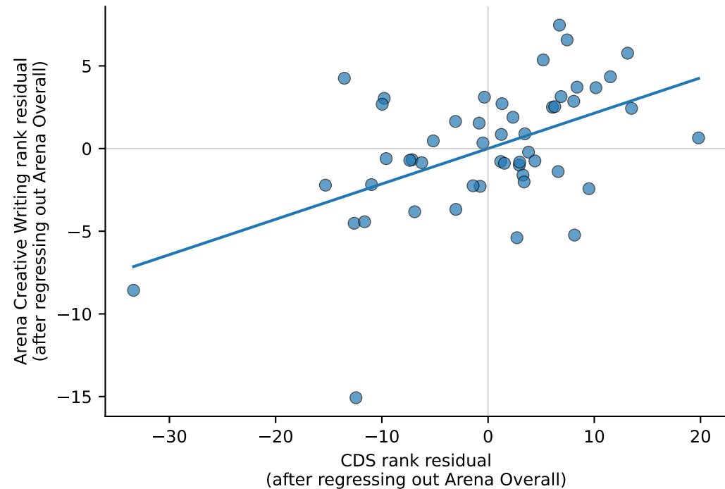
CDS vs Arena Creative Writing partial Spearman \rho = +0.439^{**} , n=51
