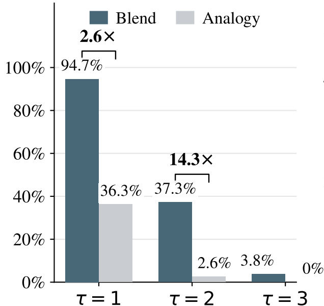
(b) Pairs in multiples by task
