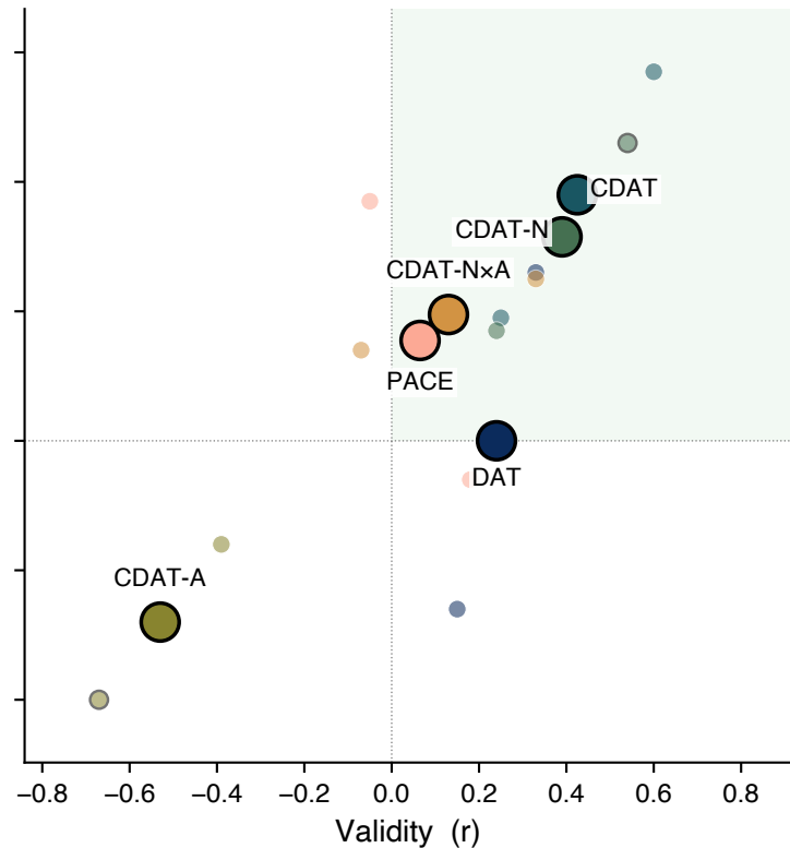
Divergent Thinking
