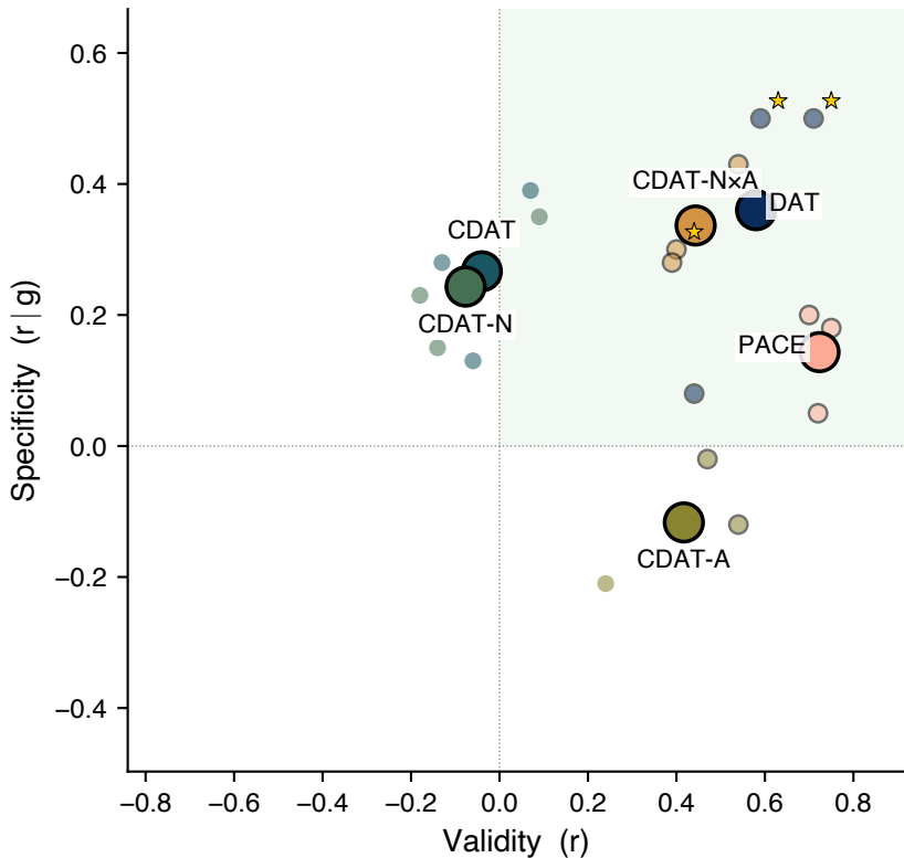
Creative Writing
