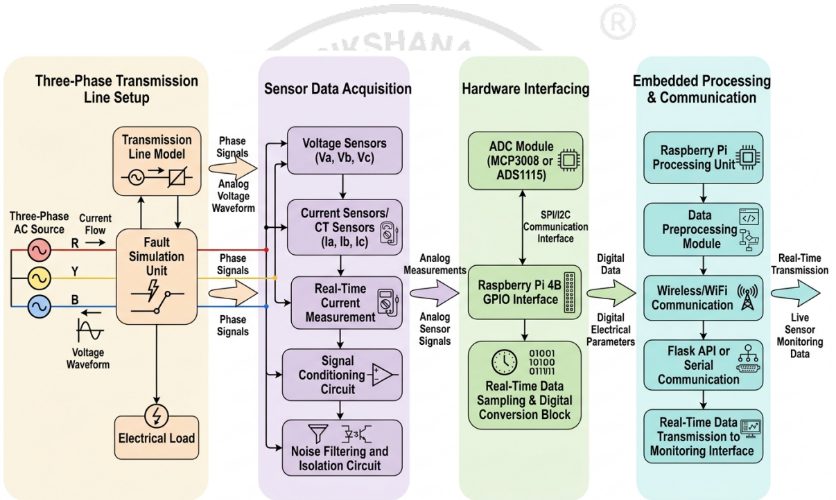
Figure 3.1: Intelligent Fault Detection and Decision Pipeline
