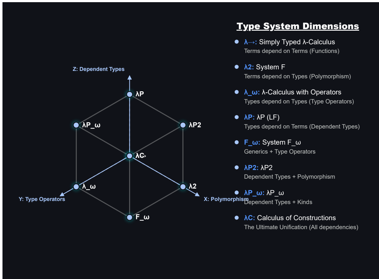
Lambda Cube
