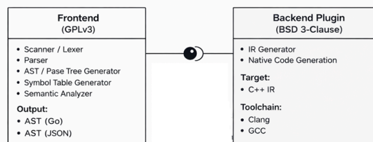
Figure: Frontend and Backend are independent components
