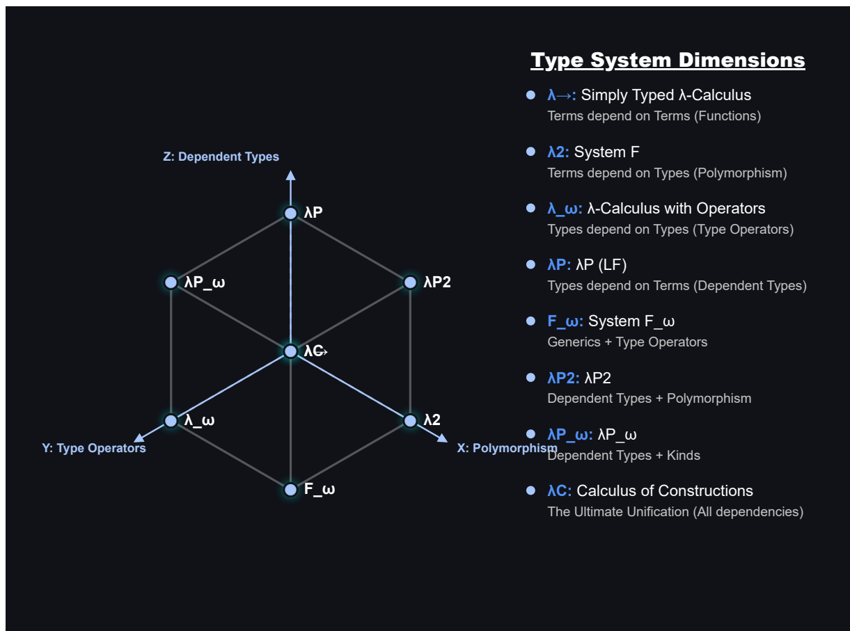
Lambda Cube
