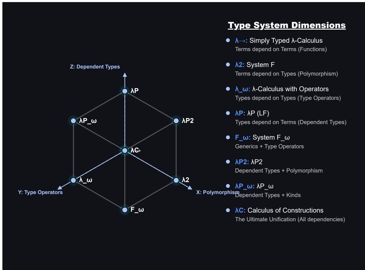
Lambda Cube
