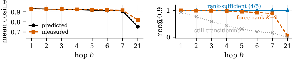
Figure 2: Recovery under repeated application of the learned matrix ( d=16 , K=8 ). Left : mean cosine for the converged seed with rank cap k=7=K-1 , compared with the prediction from its eigenspectrum alone. Right : the fraction of queries with cosine greater than 0.9, averaged over the four converged unconstrained seeds (near 1.0), and shown separately for the rank-capped seed and the fifth unconstrained seed.
