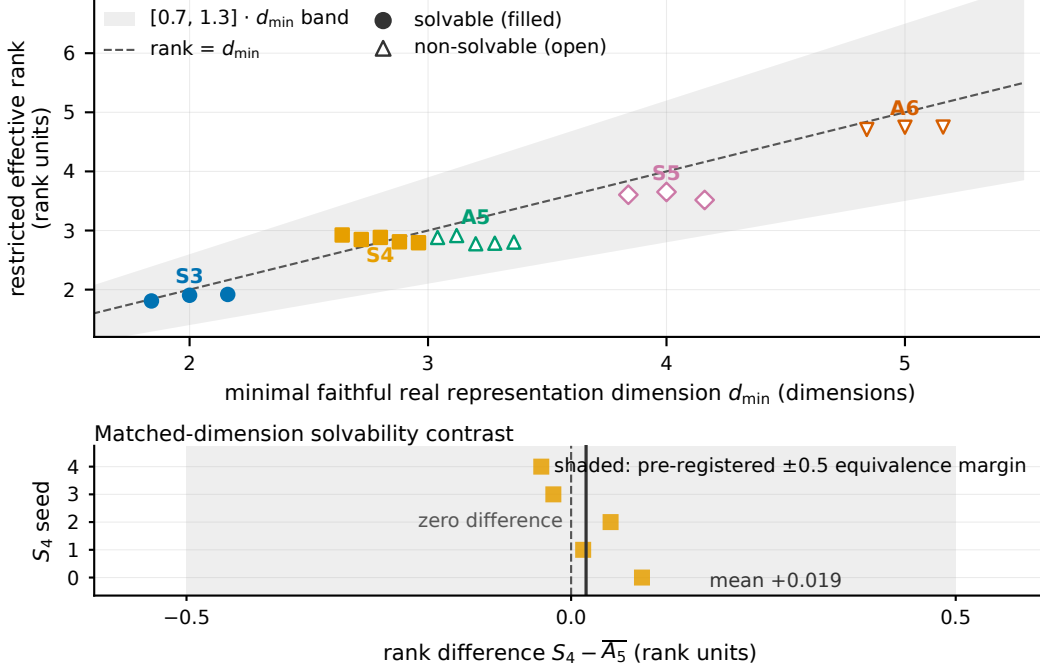
Figure 1: Recruited rank follows representation dimension across the five tested groups. Each point is one seed’s restricted effective rank on the group word problem vs. its group’s d_{\min} . Filled markers denote solvable groups; open markers denote non-solvable groups. Small horizontal offsets separate seeds at the same categorical value. Shading marks the pre-registered [0.7, 1.3] \cdot d_{\min} band, and the dashed line marks the identity. All 19 seeds are in band, and S_4/A_5 coincide at d_{\min} = 3 . The lower panel plots per-seed S_4 - A_5 rank differences at matched d_{\min} = 3 against the pre-registered \pm 0.5 rank-unit equivalence margin. Shading marks the margin. The vertical lines mark zero difference and the observed mean difference, +0.019 (Section 4).
