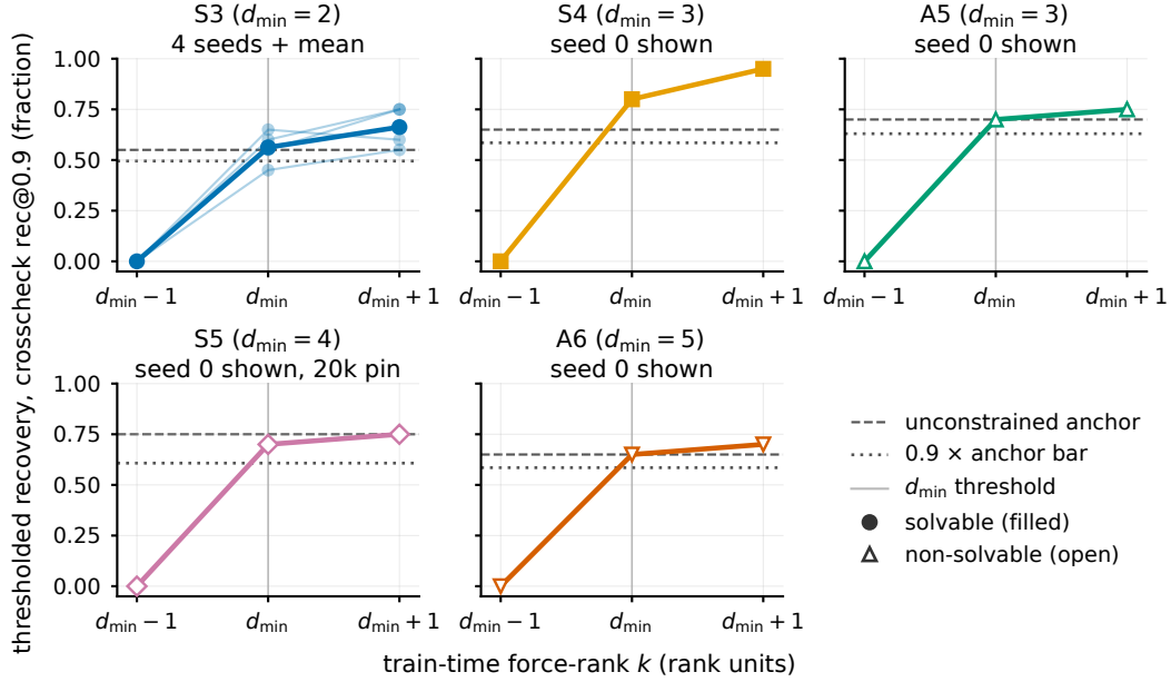
Figure 2: Recovery at a cosine-similarity threshold of 0.9 is a step function at d_{\min} : per group, crosscheck rec@0.9 on held-out words at force-rank k \in \{d_{\min}-1, d_{\min}, d_{\min}+1\} , vs. the unconstrained anchor (dashed) and the 0.9 \times anchor bar (dotted). S_3 overlays its four seeds (thin lines; bold mean); its below- d_{\min} zero is unanimous. The other four groups are drawn at seed 0; their four-seed sufficiency verdicts are in Table 1. S_5 's dotted bar is its decisional bar, 0.9 \times its four-seed anchor mean at its 20k pin (Appendix F).
