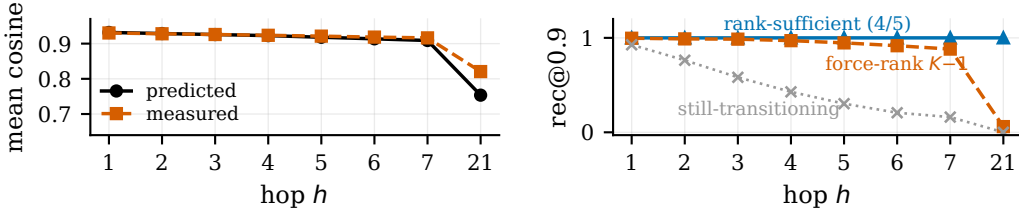
Figure 2: Recovery under repeated application of the learned matrix ( d=16 , K=8 ). Left : mean cosine for the converged seed with rank cap k=7=K-1 , compared with the prediction from its eigenspectrum alone. Right : the fraction of queries with cosine greater than 0.9, averaged over the four converged unconstrained seeds (near 1.0), and shown separately for the rank-capped seed and the fifth unconstrained seed.
