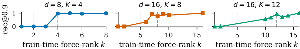
Figure 1: Recovery under training-time rank caps in the pre-registered causal test. \text{rec}@0.9 is the fraction of queries with cosine similarity greater than 0.9; the dashed line marks k = K . The archived sweep shows recovery increasing near k = K , with a more gradual transition for d=16 , K=12 .
