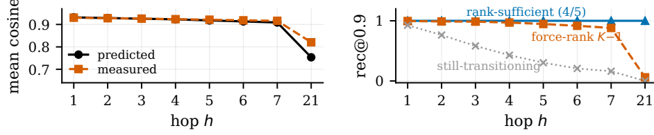
Figure 2: Depth as a spectral-exactness amplifier ( d=16 , K=8 ). Left : mean cosine for the converged force-rank k=7=K-1 seed against the eigenspectrum-only prediction (no raw keys). Right : \text{rec}@0.9 by hop for the four converged rank-sufficient seeds (flat at 1.0), the rank-starved operator, and the still-transitioning seed.
