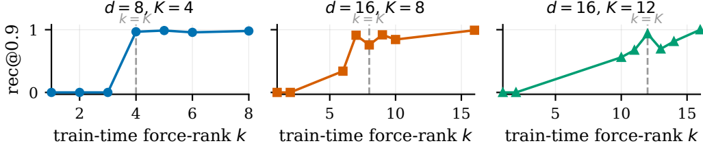
Figure 1: The primary, pre-registered causal test: \text{rec}@0.9 under train-time force-rank k (archived 991-run sweep; dashed line at k = K ). The step lands at k \approx K in every cell.
