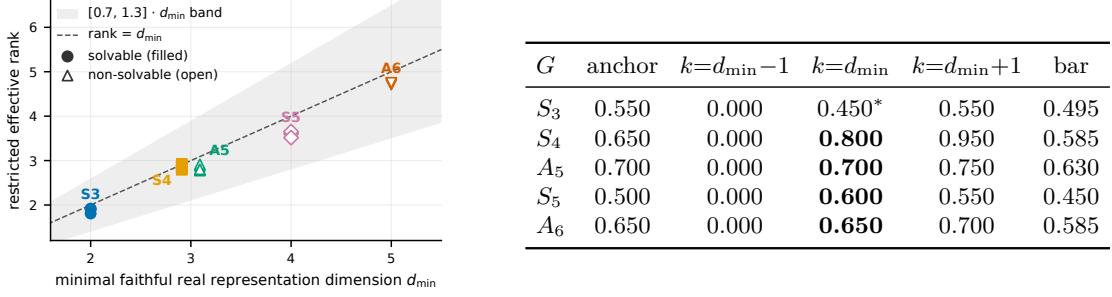
Figure 1: Left: recruited rank follows representation dimension, not solvability. Each point is one seed’s restricted effective rank vs. its group’s d_{\min} (filled: solvable; open: non-solvable); all 19 seeds are in band, and S_4/A_5 coincide at d_{\min} = 3 . Right: the causal razor on the zero-padded rank- d_{\min} target (crosscheck rec@0.9 by force-rank k , one seed per cell, unconstrained anchor, pre-registered 0.9 \times anchor bar): exactly 0.000 one rank below d_{\min} everywhere (the forced ceiling is \leq 0.894 ), clears the 0.9 \times anchor bar at d_{\min} in all five groups (bold; S_3 via seed-mean, asterisked). *extended to four seeds under the pre-stated \pm 0.05 trigger: seed-mean 0.5625 clears the fixed 0.495 bar.
