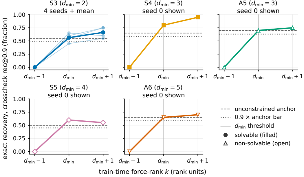
Figure 2: Exact recovery is a step function at d_{\min} . For each group, the plot reports crosscheck \text{rec}@0.9 on held-out words at force-rank k \in \{d_{\min}-1, d_{\min}, d_{\min}+1\} . Dashed lines mark the unconstrained anchor, dotted lines mark the 0.9 \times anchor bar, and gray vertical lines mark the group threshold. Filled markers denote solvable groups; open markers denote non-solvable groups. S_3 overlays its four seeds (thin marked lines; bold mean); its below- d_{\min} zero is unanimous. The plot draws the other four groups at seed 0; Table 1 gives their four-seed sufficiency verdicts, and S_5 fails at n = 4 .
