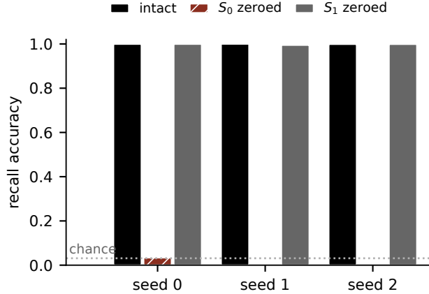
Figure 2: Causal state-zeroing on the matrix fast-weight model, per seed on the primary cell (4,096 pinned queries per read; chance 1/32). Zeroing the first block’s fast-weight state S_0 before the query continuation collapses recall to chance; zeroing the second block’s state S_1 leaves it within noise of intact. The bindings are causally resident in S_0 .
