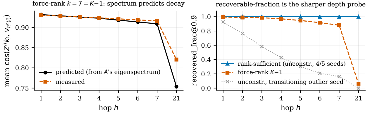
Figure 2: [Primary, pre-registered – Table 3 in figure form, plus the rank-sufficient contrast from §4.1.] Left: force-rank k=7=K-1 at K=8 – the spectral prediction (no raw keys, §4.2) against the measured curve, at every archived hop (not only the five in Table 3). Right: the behavioral contrast that motivates using recovered_frac@0.9 over mean cosine as the primary metric – rank-sufficient seeds (mean of the 4/5 converged unconstrained-rank seeds) stay flat at 1.00 through h=21 , force-rank K-1 collapses, and the fifth (still-transitioning) unconstrained-rank seed shows the same decay signature, consistent with §4.1’s reading that it is mid-transition rather than a new failure mode.
