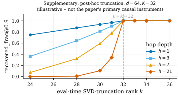
Figure 4: [Supplementary / illustrative – not one of this paper’s pre-registered claims and not behind any table in the main text.] A different causal instrument from this paper’s primary test (Figure 1, which forces rank at train time): here a single unconstrained-rank d=64, K=32 operator is trained once, then truncated to rank k post hoc at eval time via SVD, and re-scored at several hop depths. We include it only because it is a strikingly clean picture of the same underlying mechanism – a knee at k=K that sharpens with composition depth h – at an operating point an order of magnitude larger than Table 2’s cells. It is not evidence for this paper’s causal claim on its own terms: Task D’s own M2 eval-time-truncation probe was informative there only because M3’s train-time force-rank result was pre-registered as primary (§2.5); post-hoc truncation alone was the uninformative instrument in the companion paper’s CODI setting (§1). Read this figure as a mechanism illustration, not as a fourth confirmed cell of Table 5 – its (d, K) = (64, 32) operating point and step budget do not match any row of that table.
