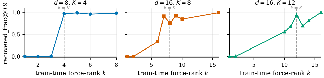
Figure 1: [Primary, pre-registered causal result – Table 2 in figure form.] recovered_frac@0.9 under train-time force-rank k (control C1, §2.5), for all three tested (d, K) cells, showing the full archived grid (the table omits some intermediate k for space). The step lands at k \approx K (dashed line) in every cell; note the d=8, K=4 knee is razor-sharp while d=16, K=12 already shows a ragged, non-monotonic transition near k \approx K in this (991-run-snapshot) data – consistent with, though numerically distinct from, the separately-reported 1,234-run mega-replication’s refined ramp in Table 2’s caption. Regenerated directly from the 991-run archived snapshot (figures/make_figures.py), not re-typed from the table.
