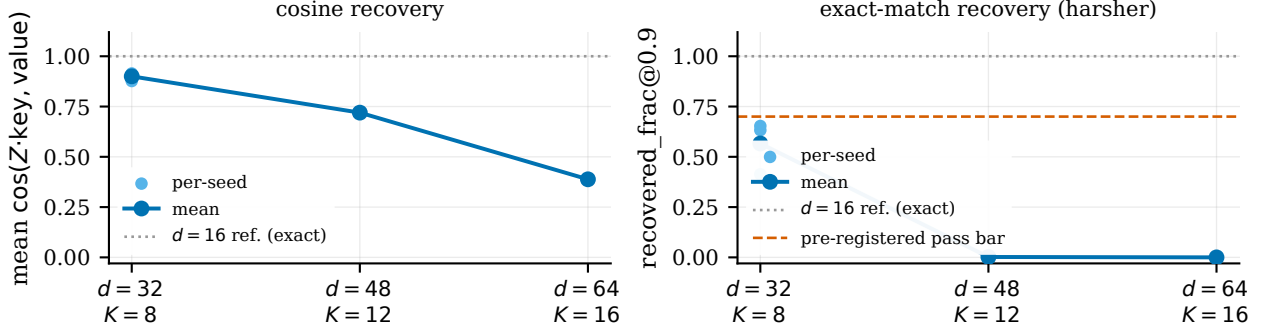
Figure 3: [Primary, pre-registered – Table 5 in figure form.] The K=d/4 exactness frontier at fixed encoder width h=64 , both by cosine (left) and by the harsher exact-match recovered_frac@0.9 (right, with the pre-registered > 0.7 formal pass bar). Individual seeds are shown where more than one was run ( d=32 ); d=48, 64 are single confirmed-flat seeds, per §5.2. The d=16 reference line marks the earlier, exact regime (§3–4) for scale; it is not a new data point plotted here.
