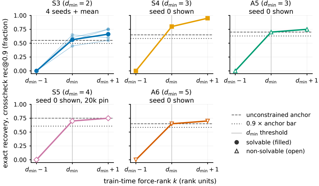
Figure 2: Exact recovery is a step function at d_{\min} : per group, crosscheck \text{rec}@0.9 on held-out words at force-rank k \in \{d_{\min}-1, d_{\min}, d_{\min}+1\} , vs. the unconstrained anchor (dashed) and the 0.9 \times anchor bar (dotted). S_3 overlays its four seeds (thin lines; bold mean); its below- d_{\min} zero is unanimous. The other four groups are drawn at seed 0; their four-seed sufficiency verdicts are in Table 1. S_5 's dotted bar is its decisional bar, 0.9 \times its four-seed anchor mean at its 20k pin (Appendix F).
