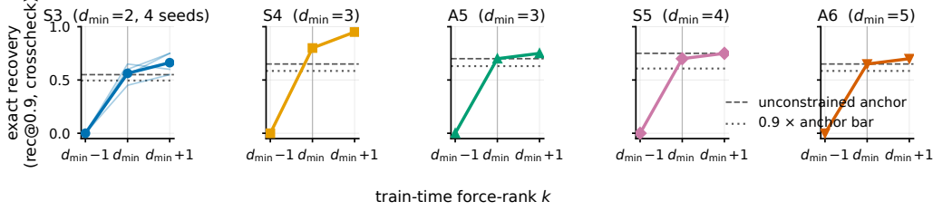
Figure 2: Exact recovery is a step function at d_{\min} : per group, crosscheck \text{rec}@0.9 on held-out words at force-rank k \in \{d_{\min}-1, d_{\min}, d_{\min}+1\} , vs. the unconstrained anchor (dashed) and the 0.9 \times anchor bar (dotted). S_3 overlays its four seeds (thin lines; bold mean); its below- d_{\min} zero is unanimous. The other four groups are drawn at seed 0; their four-seed sufficiency verdicts are in Table 1. S_5 's dotted bar is its decisional bar, 0.9 \times its four-seed anchor mean at its 20k pin (Appendix F).
