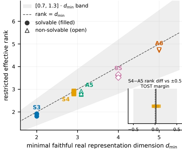
Figure 1: Recruited rank follows representation dimension, not solvability. Each point is one seed’s restricted effective rank on the group word problem vs. its group’s d_{\min} (filled: solvable; open: non-solvable), with the pre-registered [0.7, 1.3] \cdot d_{\min} band and the identity line; all 19 seeds are in band, and S_4/A_5 coincide at d_{\min} = 3 . Inset: per-seed S_4 - A_5 rank differences at matched d_{\min} = 3 against the pre-registered \pm 0.5 rank-unit equivalence margin (shaded); the vertical line is the observed mean difference, +0.019 (Section 4).
