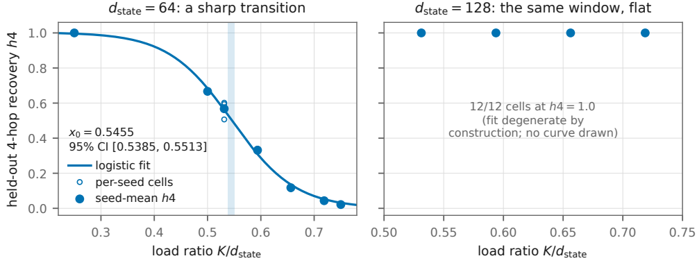
Figure 1: Held-out 4-hop recovery h4 (rec@0.9, exact continuous cosine, never argmax) versus load ratio K/d_{\text{state}} in a single-layer DeltaNet on the 107-entity recall grammar. Left: at d_{\text{state}} = 64 , seed-mean recovery over the measured loads ( K = 16 saturation anchor, archived K = 32/48 , new K = 34/38/42/46 at three seeds each; open circles are per-seed cells) transitions sharply; the logistic fit locates the midpoint at x_0 = 0.5455 with 95% bootstrap CI [0.5385, 0.5513] (shaded band). Right: the identical K/d_{\text{state}} window re-run at d_{\text{state}} = 128 ( K = 68/76/84/92 , three seeds each) is flat at exact ceiling, h4 = 1.0 in 12 of 12 cells; the sigmoid fit on this flat data is degenerate by construction (bootstrap degenerate fraction 1.0) and no curve is drawn, per the pre-registered disclosure rule. Takeaway: the same load ratio that collapses recall at d_{\text{state}} = 64 is loss-free at d_{\text{state}} = 128 .
