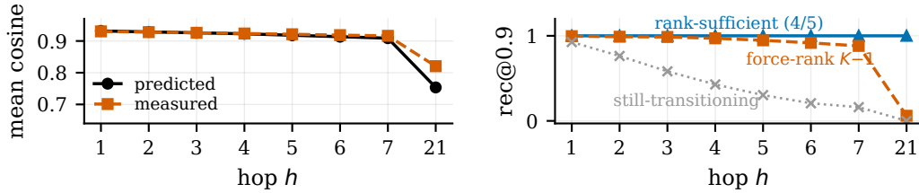
Figure 2: Depth as a spectral-exactness amplifier ( d=16 , K=8 ). Left : mean cosine for the converged force-rank k=7=K-1 seed against the eigenspectrum-only prediction (no raw keys). Right : \text{rec}@0.9 by hop for the four converged rank-sufficient seeds (flat at 1.0), the rank-starved operator, and the still-transitioning seed.
