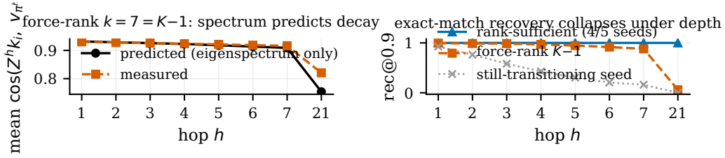
Figure 2: Depth as a spectral-exactness amplifier ( d=16, K=8 ). Left : mean cosine for the converged force-rank k=7=K-1 seed against the eigenspectrum-only prediction (no raw keys). Right : \text{rec}@0.9 by hop for the four converged rank-sufficient seeds (flat at 1.0), the rank-starved operator, and the still-transitioning seed.
