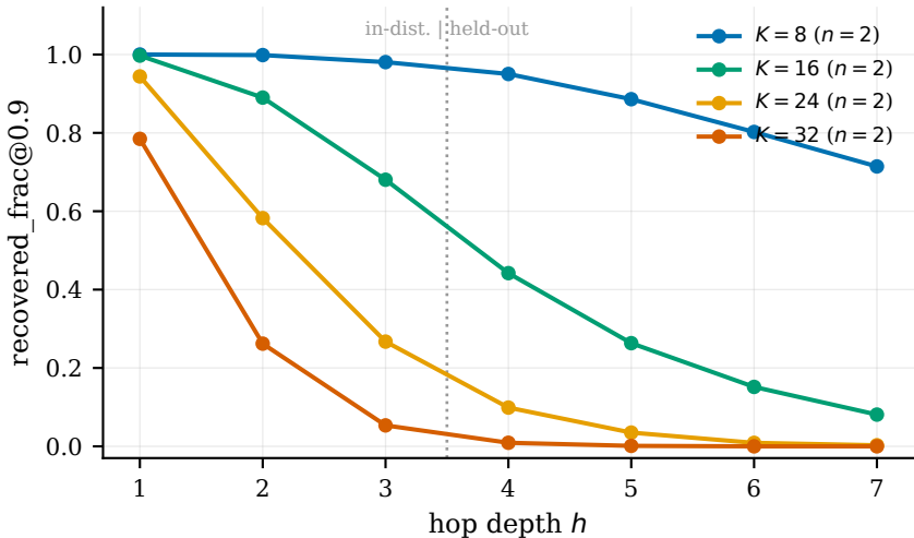
Real-text K-axis exactness frontier ( d_{\text{state}} = 64 , waveA, per-seed mean)
