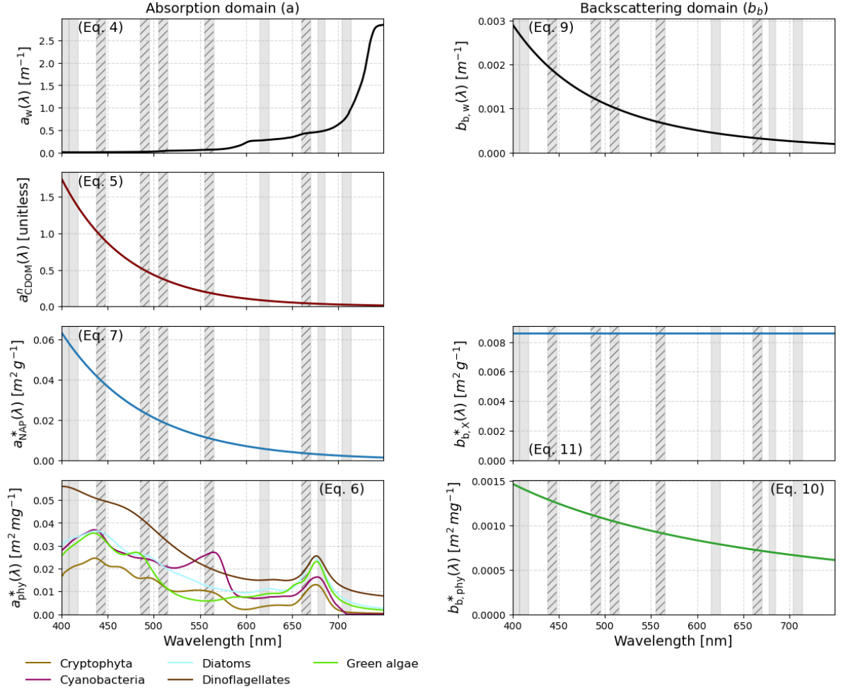
Figure 5: IOPs and SIOPs as configured with the Lake Constance pre-sets from Table 6. Reference to the Equations is given in brackets. Grey bars indicate Sentinel-3 OLCI wavelengths (full width at half maximum), hatched bars signify the used bands. From Equation 4: Absorption of pure water; note that a_{w,T}(\lambda) equals a_w(\lambda) given T = 20^\circ . From Equation 9: Backscattering of pure water. From Equation 5: Normalized absorption coefficient of CDOM (exponential approximation). From Equation 7: Specific absorption coefficient of NAP. From Equation 11: Specific backscattering coefficient of NAP. From Equation 6: Normalized absorption coefficient of phytoplankton. From Equation 10: Normalized backscattering coefficient of phytoplankton.
