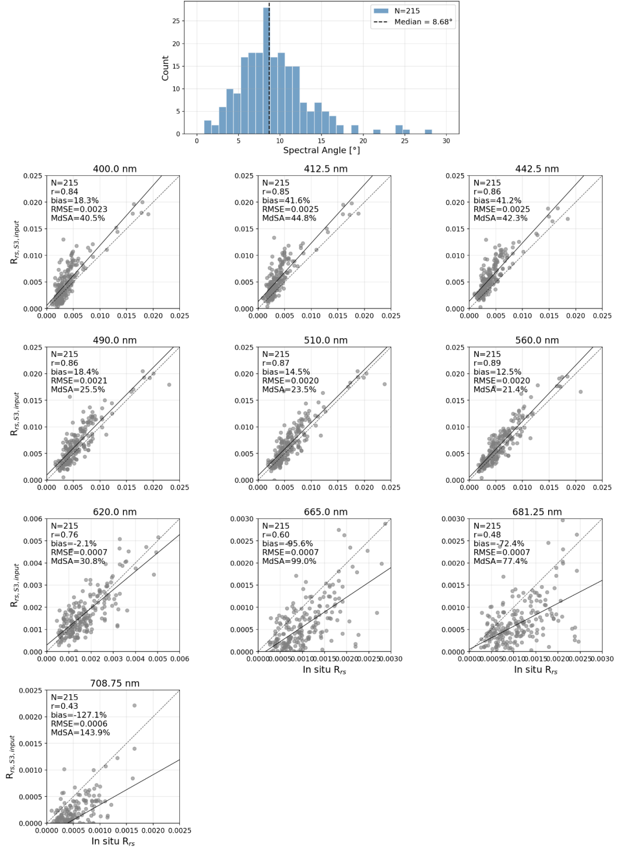
Figure 7: Validation of the atmospheric correction applied to the Sentinel-3 imagery, at all available bands. Top: histogram of the spectral angle between the atmospherically corrected and in situ reflectance spectra. Below: one scatter plot per band, comparing the atmospherically corrected Sentinel-3 remote sensing reflectance ( R_{rs,S3,input} ) against the in situ remote sensing reflectance ( R_{rs} ) at the same wavelength, with the 1:1 line (dashed) and best fit (solid). Axis bounds differ between panels.
