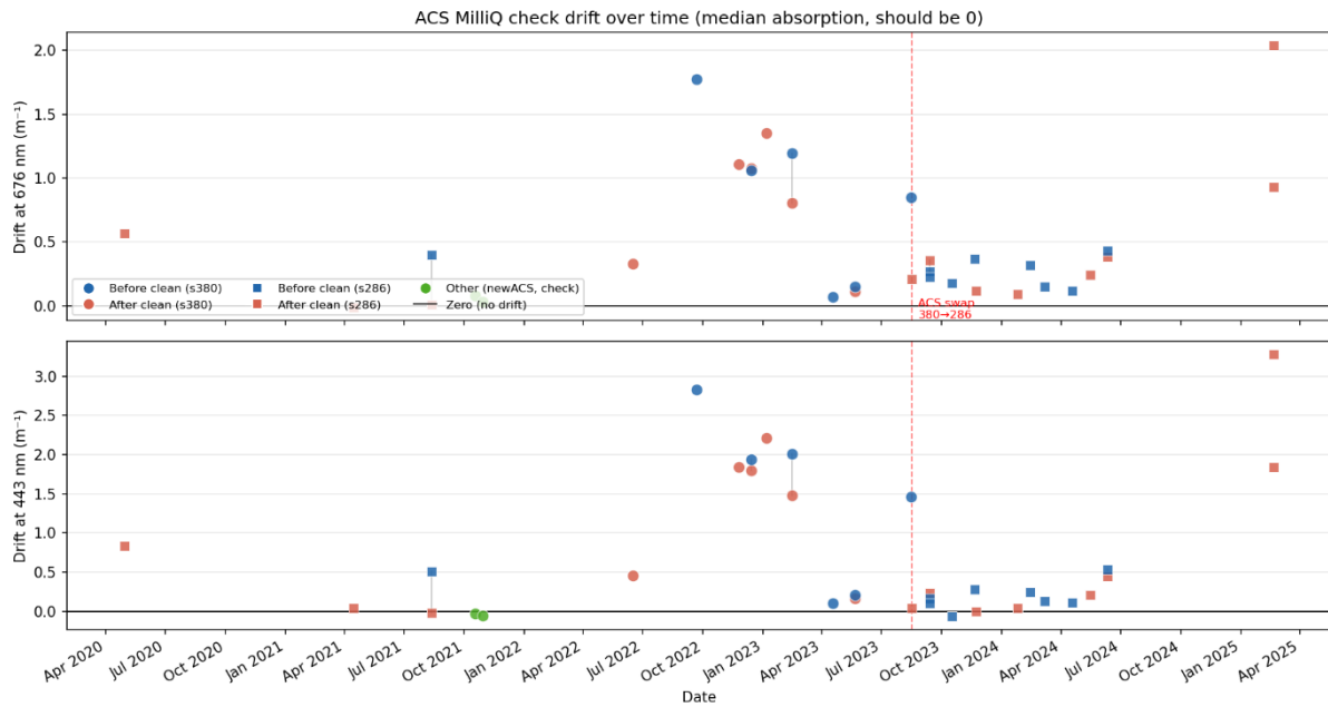
Figure A5. 1: Drift of the AC-S instrument absorption measurements at Thetis. An AC-S instrument switch is indicated in 2023. Courtesy of Jonas Wydler.
