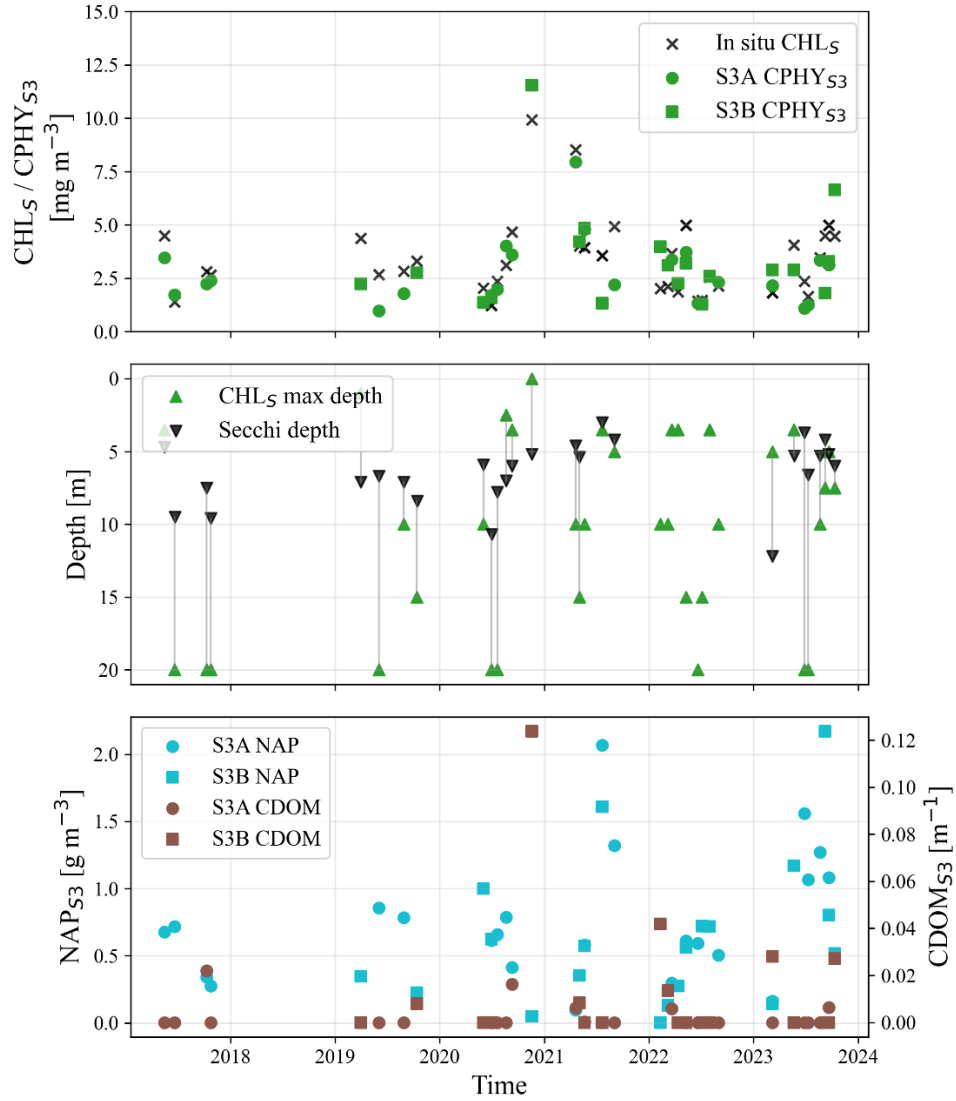
Figure 10: Time series at the SHL2 monitoring station, 2017 – 2024. Top: satellite-modeled phytoplankton concentration from Sentinel-3A and 3B (S3A and S3B; CPHY_{53} ) against in situ spectrophotometric chlorophyll a ( CHL_5 ). Middle: depth of the CHL_5 maximum compared with the Secchi disk depth (the depth to which the water is visually transparent). Bottom: satellite-modeled non-algal particle concentration ( NAP_{53} ) and colored dissolved organic matter absorption ( CDOM_{53} ) over time.
