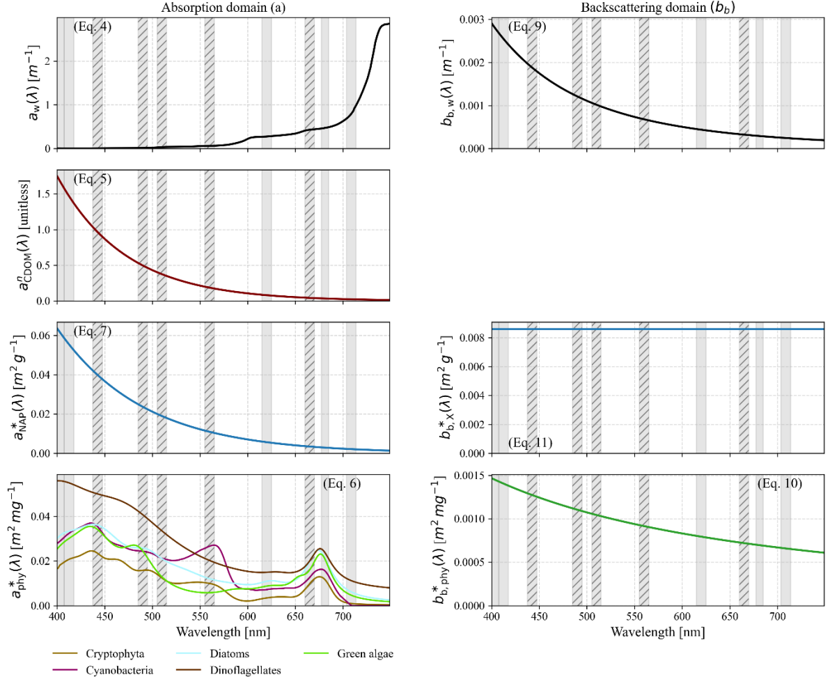
Figure 5: (Specific) inherent optical properties as configured with the pre-sets from Table 6. Reference to the Equations is given in brackets. Grey bars indicate Sentinel-3 OLCI wavelengths (full width at half maximum), hatched bars signify the used bands. From Equation 4: Absorption of pure water; note that a_{w,T}(\lambda) equals a_w(\lambda) given T = 20^\circ . From Equation 9: Backscattering of pure water. From Equation 5: Normalized absorption coefficient of CDOM (exponential approximation). From Equation 7: Specific absorption coefficient of NAP. From Equation 11: Specific backscattering coefficient of NAP. From Equation 6: Normalized absorption coefficient of phytoplankton. From Equation 10: Normalized backscattering coefficient of phytoplankton.
