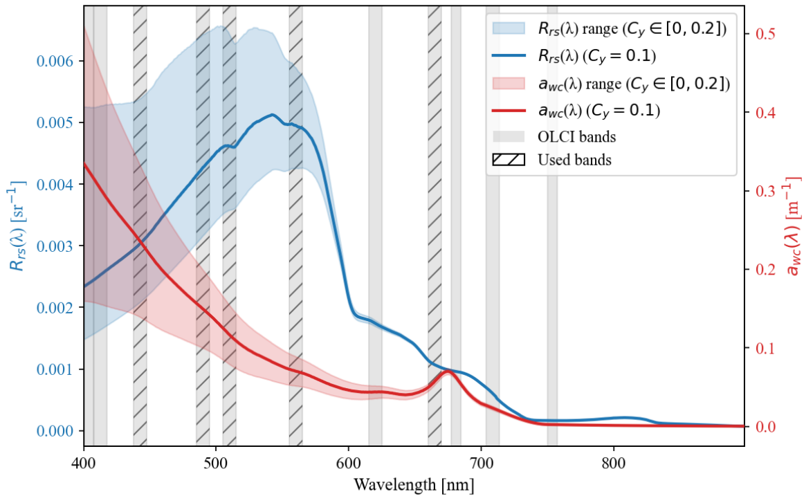
Figure 25: WASI forward-modeled remote sensing reflectance ( R_{rs}(\lambda) ) and constituent absorption ( a_{wc}(\lambda) ) for “standard” Lake Geneva concentrations ( C_0 = 3 \text{ mg m}^{-3} , C_X = 1 \text{ g m}^{-3} ) with C_Y varying between 0 and 0.2 \text{ m}^{-1} . Grey bars indicate Sentinel-3 OLCI wavelengths (full width at half maximum); hatched bars signify the bands used for MiniWASI image inversion.
