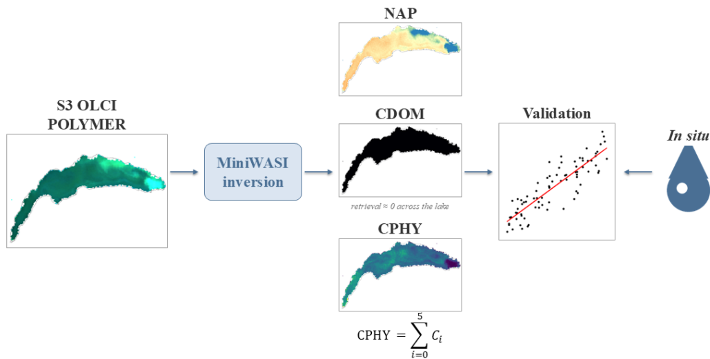
Figure 4: Schematic overview for the validation of the three basic constituents retrieved from Sentinel-3 (S3). NAP: non-algal particles, CDOM: colored dissolved organic matter, CPHY: phytoplankton concentration (sum of five classes).
