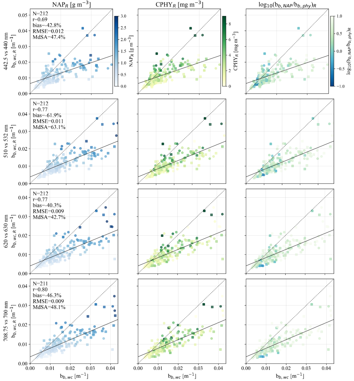
Figure A3. 1: Validation of constituent backscattering modeled from hyperspectral in situ R_{rs}(\lambda) at the four wavelength pairs used for satellite validation (442.5 vs. 440, 510 vs. 532, 620 vs. 630, and 708.75 vs. 700 nm). b_{b,wc,R}(wvl) : constituent backscattering as inverted from hyperspectral in situ R_{rs}(\lambda) at wavelength "wvl". b_{b,wc}(wvl) : constituent backscattering from in situ scattering conversion at wavelength "wvl". The first column is colored by non-algal particle concentration inverted from hyperspectral in situ R_{rs}(\lambda) ( NAP_R ), the second by phytoplankton concentration inverted from hyperspectral in situ R_{rs}(\lambda) ( CPHY_R ), the third by the ( \log -scale) proportion of retrieved NAP backscattering ( b_{b,NAP} ) to retrieved phytoplankton backscattering ( b_{b,phy} ). The 1:1 line (dashed) and best fit (solid) are shown in each panel; note that panels use different axis bounds.
