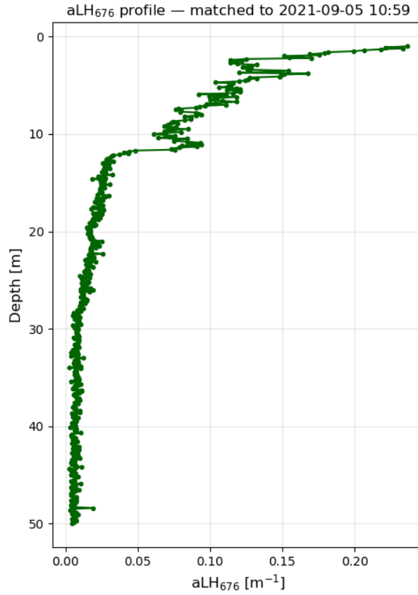
Figure A4. 1: aLH 676 profile on 5.9.2021, corresponding to a bloom of Uroglena sp. Note the strong non-uniform vertical distribution, including in the range (0-5 m) used as average for in situ references. While near surface aLH 676 is approximately 0.2 m -1 (corresponding to CHL ~ 15 mg m -3 when converted using Equation 2), it decreases to approximately 0.1 m -1 at a depth of 5 m (CHL ~ 7.5 mg m -3 ).
