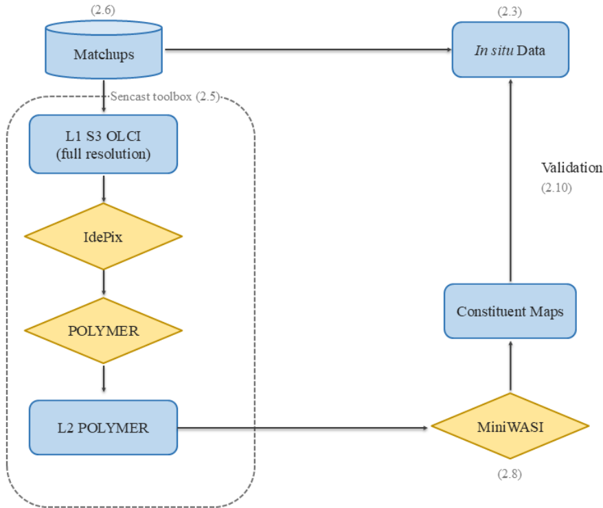
Figure 6: Schematic diagram of the processing chain presented in Section 2. References for the specific Section are given in brackets. L1: Level 1, L2: Level 2, S3: Sentinel-3, OLCI: Ocean and Land Color Instrument.
