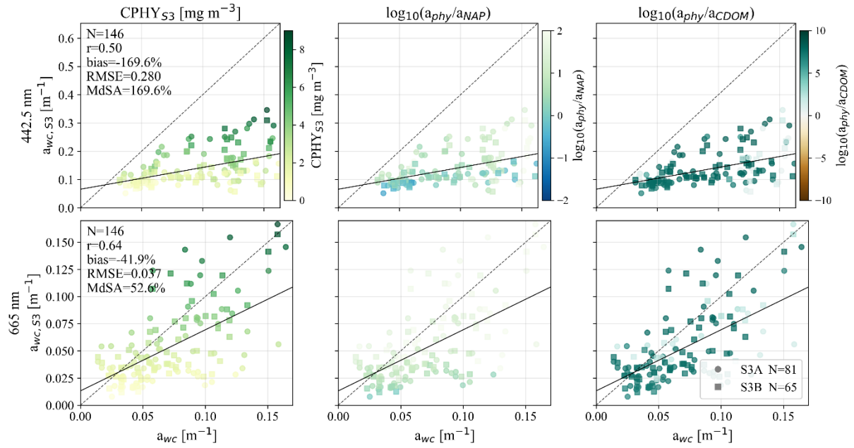
Figure 18: Validation of satellite-modeled constituent absorption from Sentinel-3A and 3B (S3A and S3B; a_{wc,S3} ) against the in situ measurement ( a_{wc} ), at the wavelengths corresponding to the phytoplankton absorption peaks used in the MiniWASI inversion (442.5 and 665 nm). Left column: points colored by the satellite-modeled phytoplankton concentration ( CPHY_{S3} ). Middle column: points colored by the (log-scale) ratio of retrieved phytoplankton absorption ( a_{phy} ) to retrieved non-algal particle absorption ( a_{NAP} ). Right column: points colored by the (log-scale) ratio of a_{phy} to retrieved colored dissolved organic matter absorption ( a_{CDOM} ). The 1:1 line (dashed) and best fit (solid) are shown in each panel; note that rows use different axis bounds.
