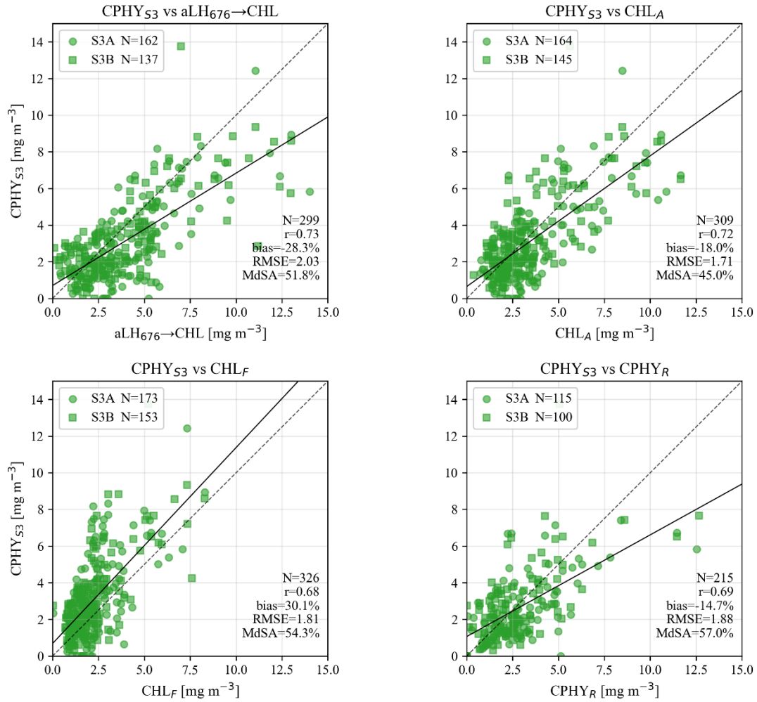
Figure 14: Validation of the satellite-modeled phytoplankton concentration from Sentinel-3A and 3B (S3A and S3B; CPHY_{S3} ) against four in situ chlorophyll a / phytoplankton references at LÉXPLORE: the absorption line height at 676 nm converted to a chlorophyll-equivalent concentration ( aLH_{676} \rightarrow CHL ), absorption-corrected chlorophyll a ( CHL_A ), fluorometric chlorophyll a ( CHL_F ), and phytoplankton concentration modeled from hyperspectral in situ reflectance ( CPHY_R ). S3A and S3B matchups are shown as circles and squares respectively. The dashed line corresponds to the 1:1 line and the solid line to the best fit. One CPHY_R matchup falls outside the plotted range.
