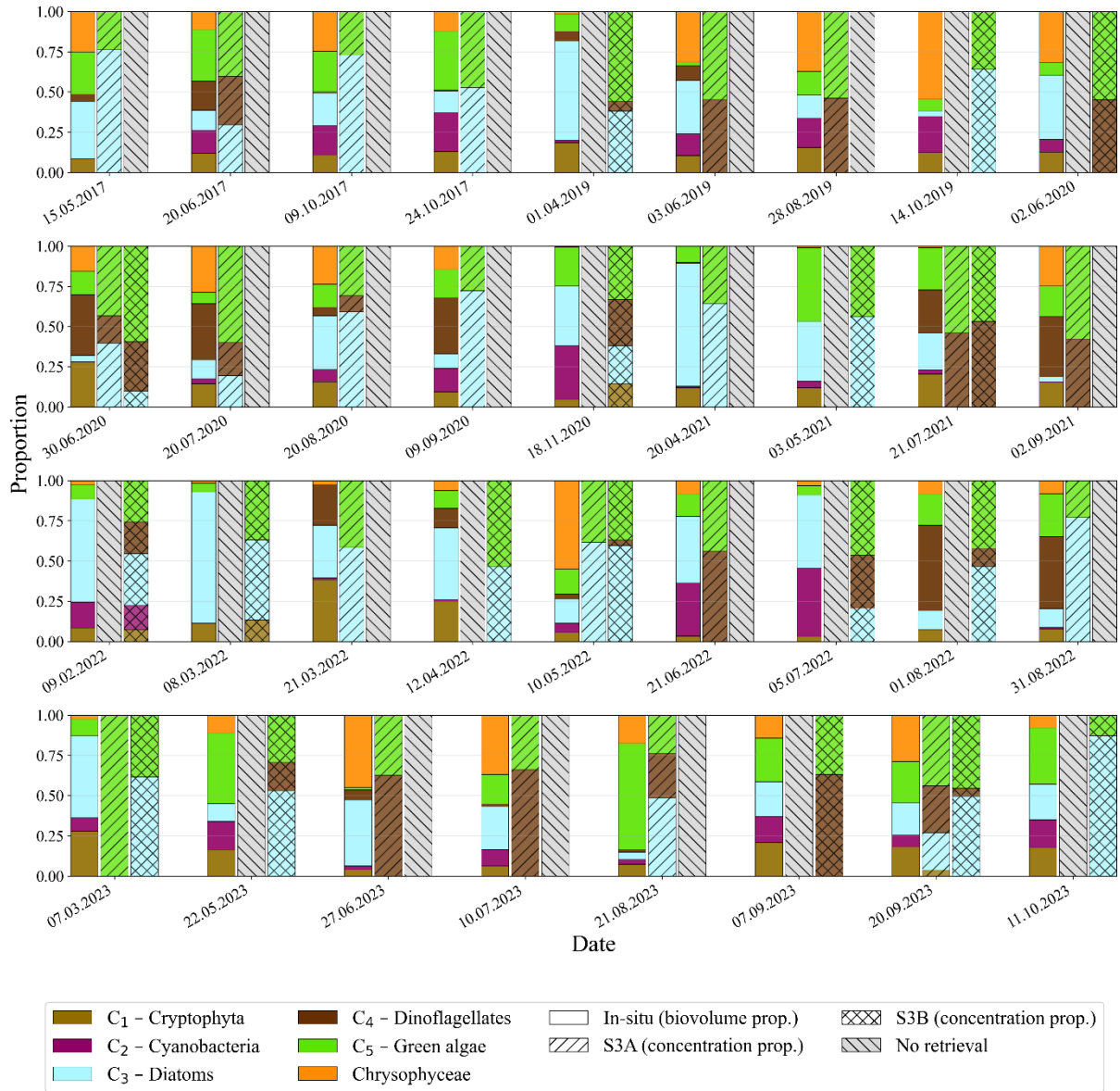
Figure 11: Relative proportions of the five phytoplankton taxa groups retrieved by the MiniWASI bio-optical inversion model from Sentinel-3A and 3B (S3A and S3B), i.e. cryptophyta ( C_1 ), cyanobacteria ( C_2 ), diatoms ( C_3 ), dinoflagellates ( C_4 ), and green algae ( C_5 ), compared with the relative in situ biovolume proportions of the same taxa, for each sampling date. In situ chrysophyceae is shown for context but is not one of the taxa parametrized by MiniWASI. Bar shading distinguishes the in situ biovolume proportion from the S3A- and S3B-modeled concentration proportions; hatched grey bars mark dates without a valid retrieval.
