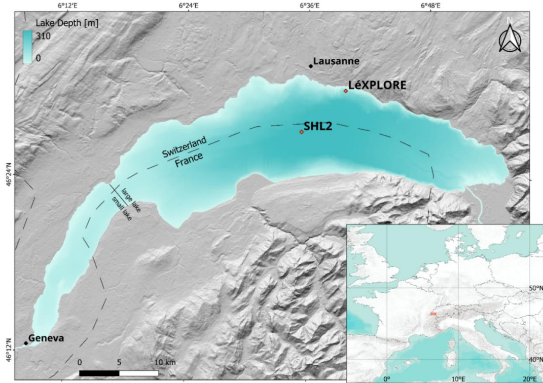
Figure 3: Overview map of Lake Geneva, including the location of the sampling station SHL2 and the LéXPLORE platform. The background hillshade and bathymetry maps are derived from the Shuttle Radar Topography Mission digital elevation model (©NASA) and swissBATHY3D datasets respectively (©swisstopo). The simplified country border is from Huwise Hub (©Huwise, OGL).
