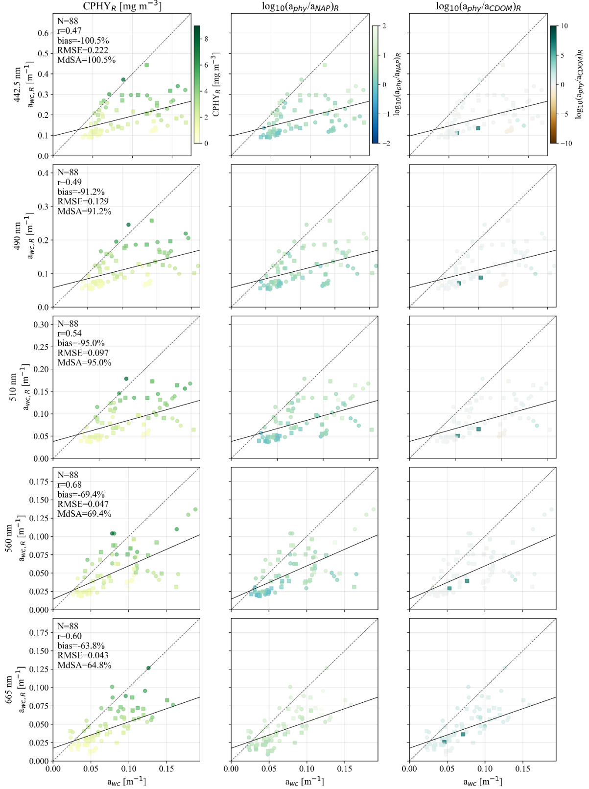
Figure A3. 2: Validation of water constituent absorption modeled from hyperspectral in situ R_{rs}(\lambda) at the five wavelengths used during inversion (442.5, 490, 510, 560, and 665 nm). a_{wc} : absorption by water constituents measured in situ, a_{wc,R} : absorption by water constituents as inverted from hyperspectral in situ R_{rs}(\lambda) . The first column is colored by phytoplankton concentration inverted from hyperspectral in situ R_{rs}(\lambda) ( CPHY_R ), the second by the (log-scale) proportion of retrieved phytoplankton absorption ( a_{phy} ) to retrieved non-algal particle absorption ( a_{NAP} ), the third by the (log-scale) proportion of a_{phy} to retrieved colored dissolved organic matter absorption ( a_{CDOM} ). The 1:1 line (dashed) and best fit (solid) are shown in each panel; note that panels use different axis bounds.
