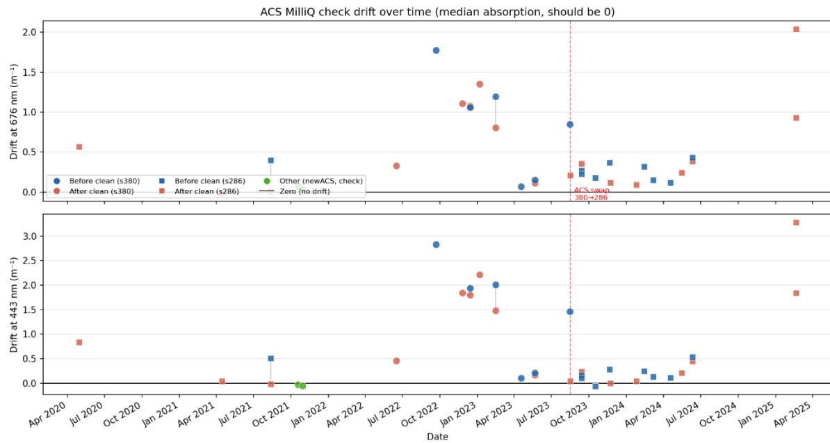
Figure A5. 1: Drift of the AC-S instrument absorption measurements at Thetis. An AC-S instrument switch is indicated in 2023. Courtesy of Jonas Wyder.
