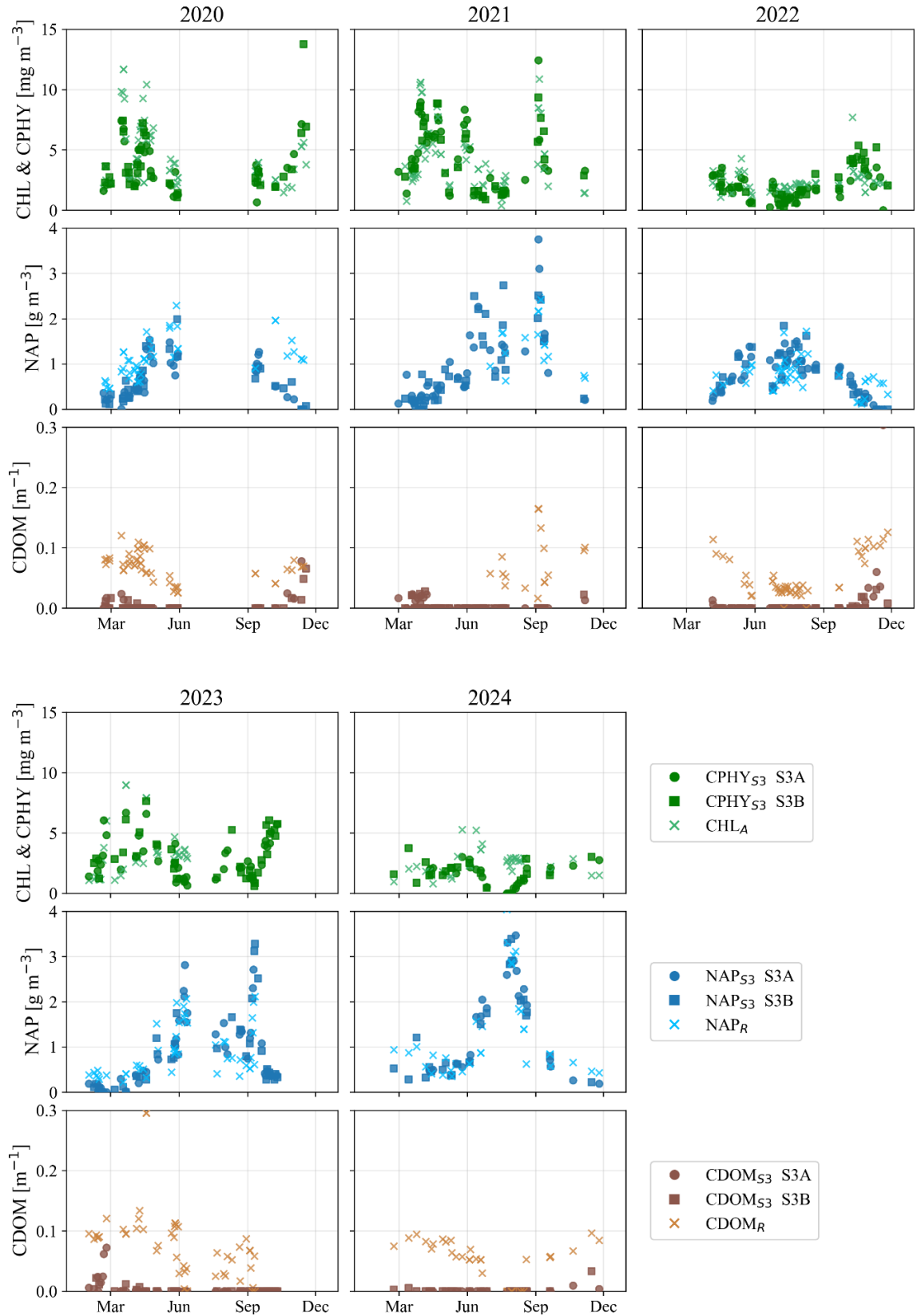
Figure 17: Time series (LéXPLORE, 2020 – 2024) of satellite and in situ water constituent estimates by year; only years with more than 10 matchups are shown. Top row: satellite-modeled phytoplankton concentration from Sentinel-3A and 3B (S3A and S3B; CPHY_{S3} ) against absorption-corrected fluorometric chlorophyll a ( CHL_A ), used here as the in situ chlorophyll a reference. Middle row: satellite-modeled non-algal particle concentration ( NAP_{S3} ) against the in situ estimate modeled from hyperspectral reflectance ( NAP_R ). Bottom row: satellite-modeled colored dissolved organic matter absorption ( CDOM_{S3} ) against the in situ estimate ( CDOM_R ).
