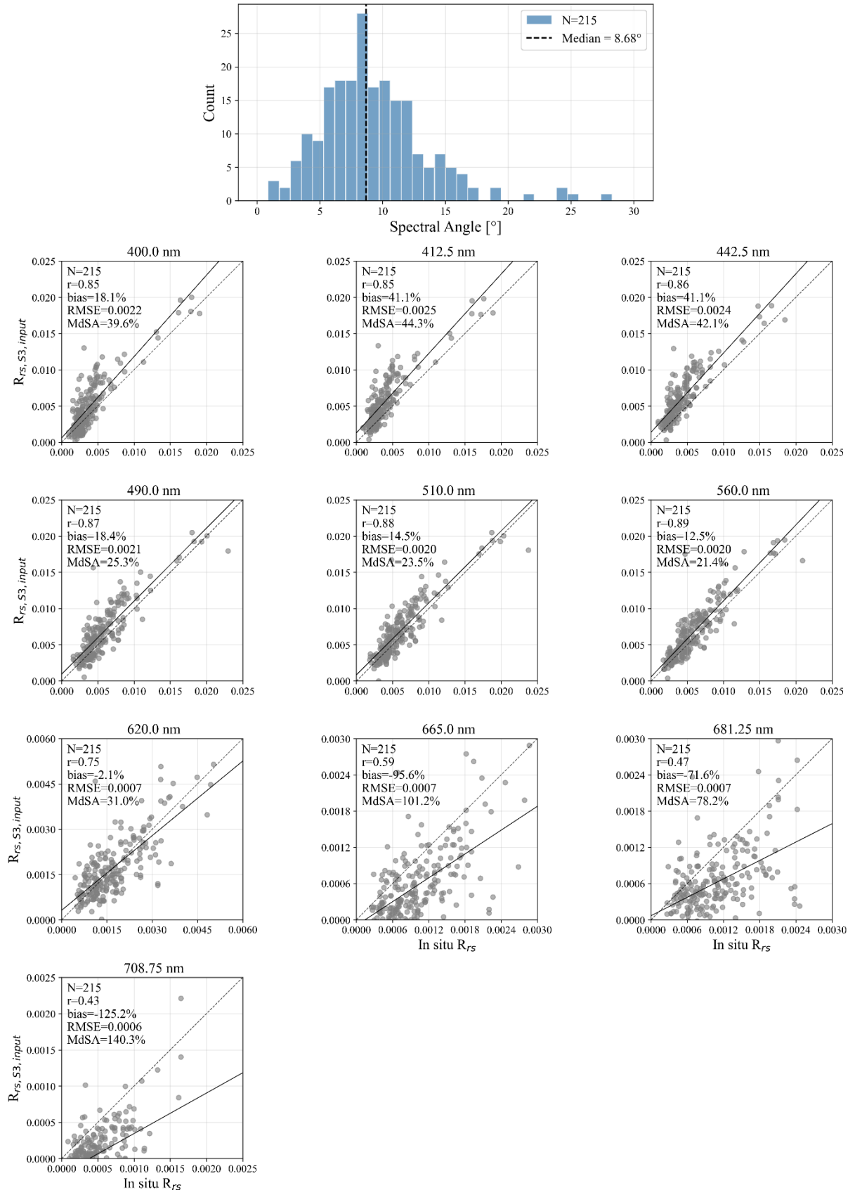
Figure 7: Validation of the atmospheric correction applied to the Sentinel-3 imagery, at all available bands. Top: histogram of the spectral angle between the atmospherically corrected and in situ reflectance spectra. Below: one scatter plot per band, comparing the atmospherically corrected Sentinel-3 remote sensing reflectance ( R_{rs,S3,input} ) against the in situ remote sensing reflectance ( R_{rs} ) at the same wavelength, with the 1:1 line (dashed) and best fit (solid). Axis bounds differ between panels.
