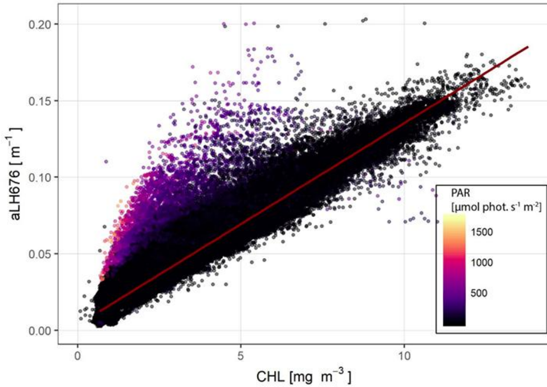
Figure A2. 1: Fluorescence-based CHL (chlorophyll a ) plotted against aLH_{676} (absorption line height at 676 nm) for the full Thetis dataset, colored by downwelling PAR (Photosynthetically Active Radiation) irradiance. The color gradient illustrates non-photochemical quenching (NPQ): as PAR rises, the CHL-to- aLH_{676} ratio declines by up to 40%, introducing bias into fluorescence-based CHL estimates under bright conditions (Minaudo et al., 2021). The red line, fit to low-PAR (nighttime) data where quenching is negligible, gives the reference relationship used in Equations 1 and 2. Reprinted from Minaudo et al., 2021, Figure S3, CC BY-NC-ND 4.0.
