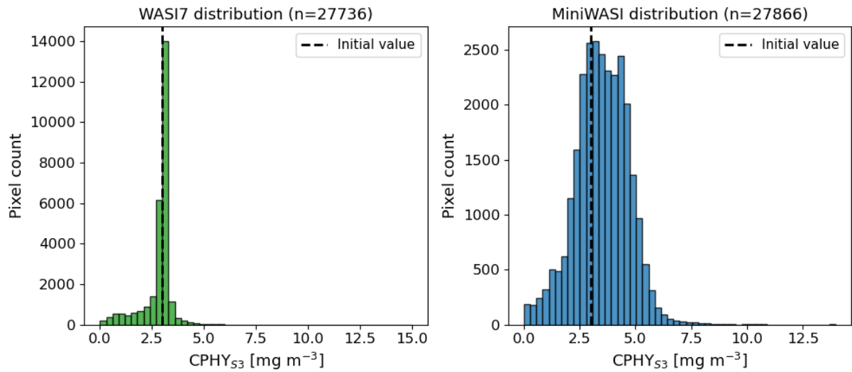
Figure A1. 3: Histograms of phytoplankton concentration values of the five campaign images (see Section 3.4; Figure A1. 1). WASI7 retrievals of phytoplankton are strongly biased towards the initial value ( 3 \text{ mg m}^{-3} ) while MiniWASI retrievals show greater variability at higher overall inversion accuracy. The number of pixels varies slightly due to the water masking procedure applied in WASI7.
