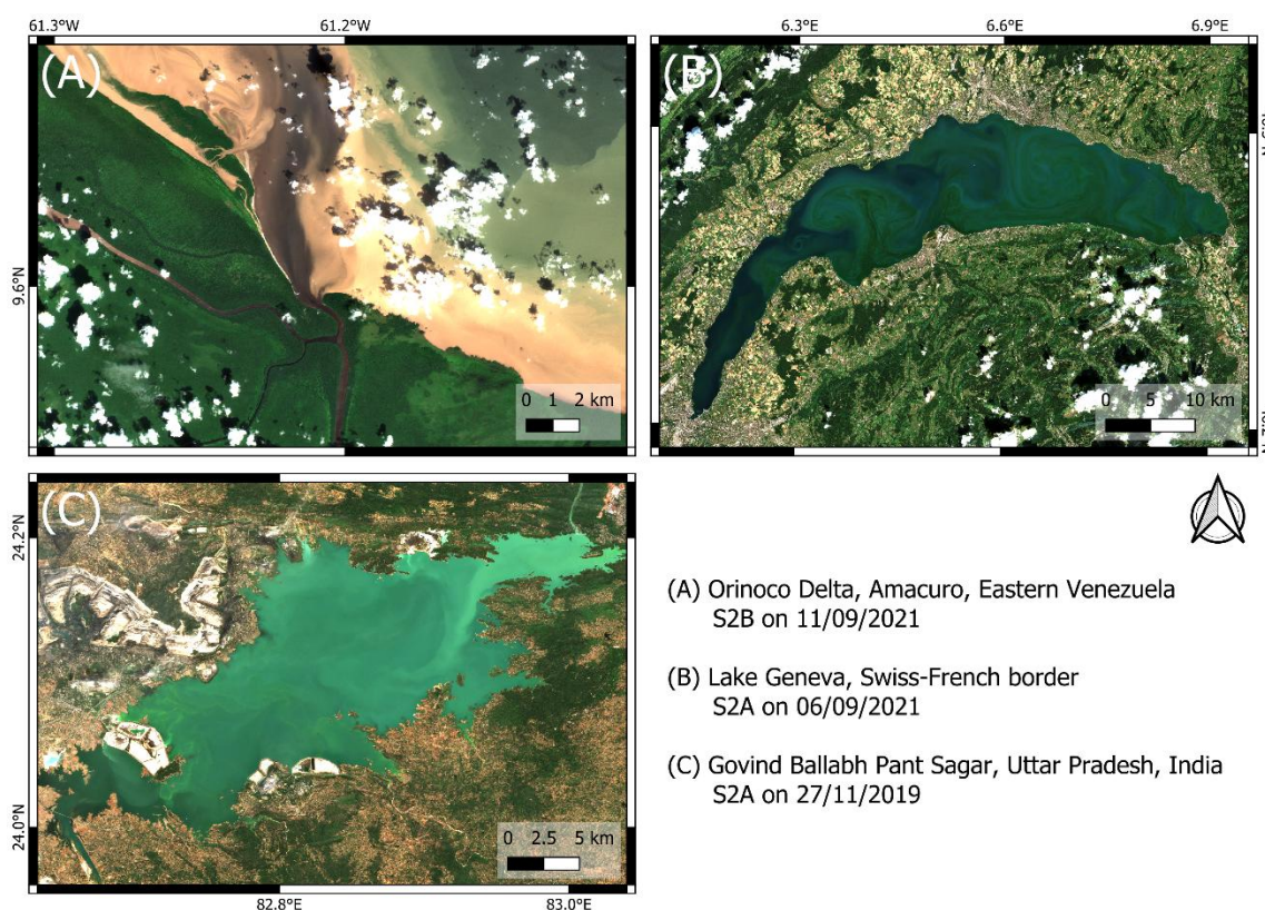
Figure 2: True-color Level 2 Sentinel-2 A/B (S2A/S2B) example images of optically active constituents in Case 2 waters, downloaded from the Copernicus browser (©Copernicus). The same scaling of the 490, 560, and 665 nm bands was applied to all images. (A) Large quantities of suspended and dissolved matter in Orinoco Delta, Eastern Venezuela (B) Bloom of Uroglena sp. phytoplankton species in Lake Geneva (C) Suspended ash particles originating from coal plants in Govind Ballabh Pant Sagar (Rihand Dam), Uttar Pradesh, India.
