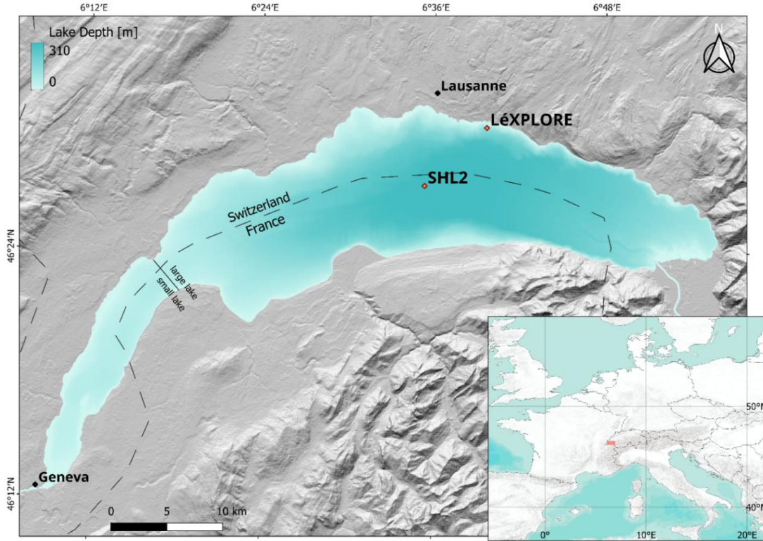
Figure 3: Overview map of Lake Geneva, including location of the sampling station SHL2 and the LÉXPLORE platform. The background hillshade and bathymetry maps are derived from the shuttle radar topography mission digital elevation model (©NASA) and swissBATHY3D datasets respectively (©swisstopo).
