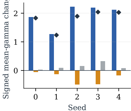
C Adam: signed gamma growth
