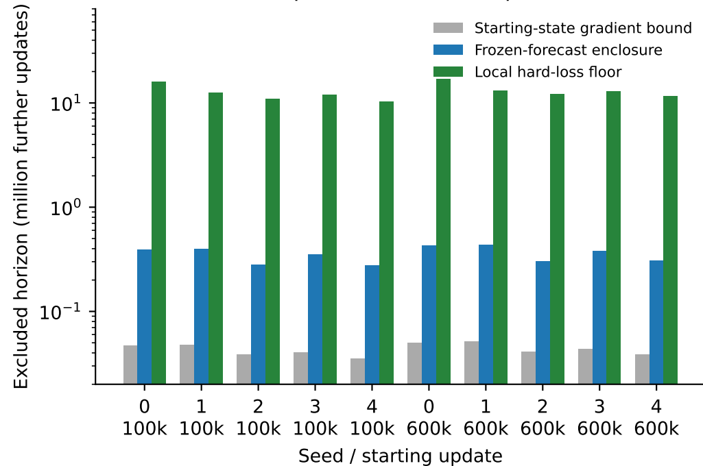
Computed exclusion of \gamma \geq 1
