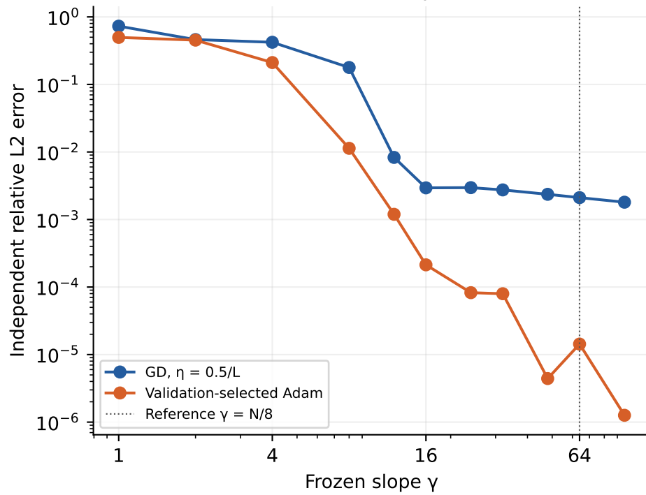
(b) Raw, 200k updates
