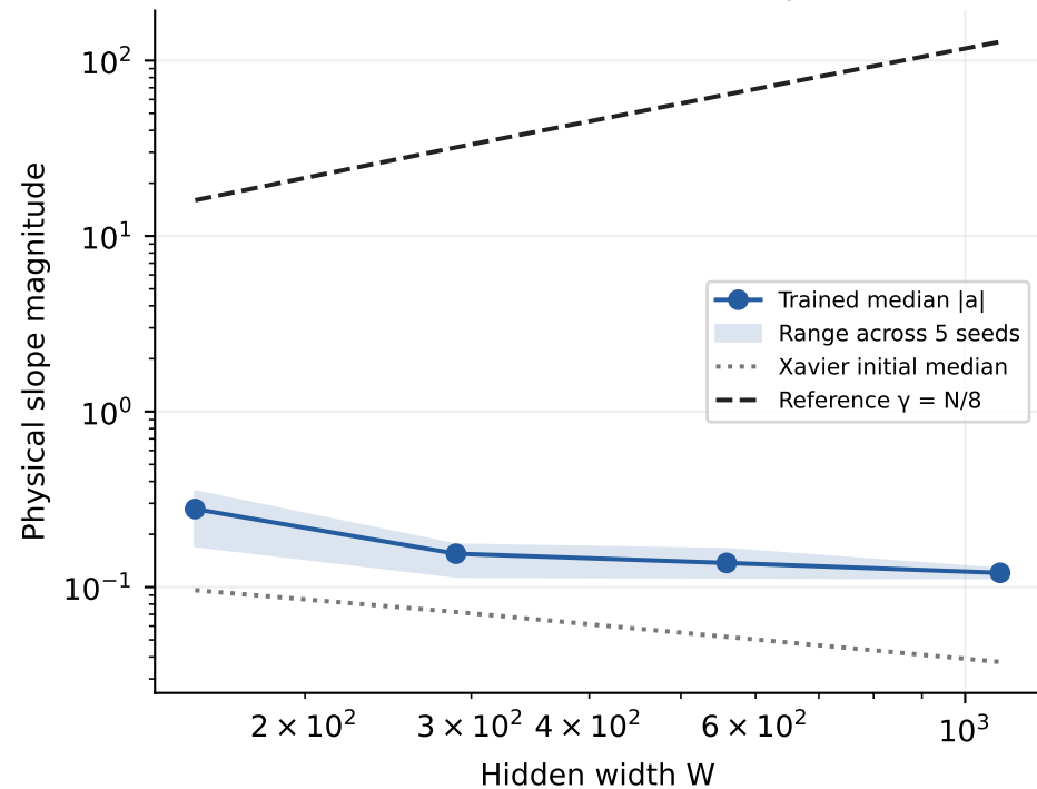
(a) End-to-end Adam, 20k updates
