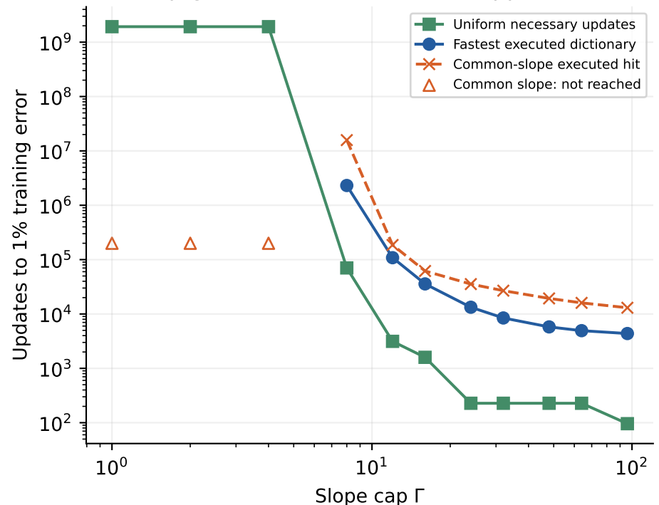
(c) Cap guarantee and executed upper witness
