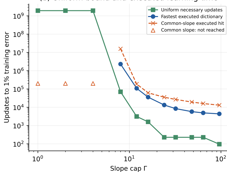
(b) Uniform bound and executed learning time
