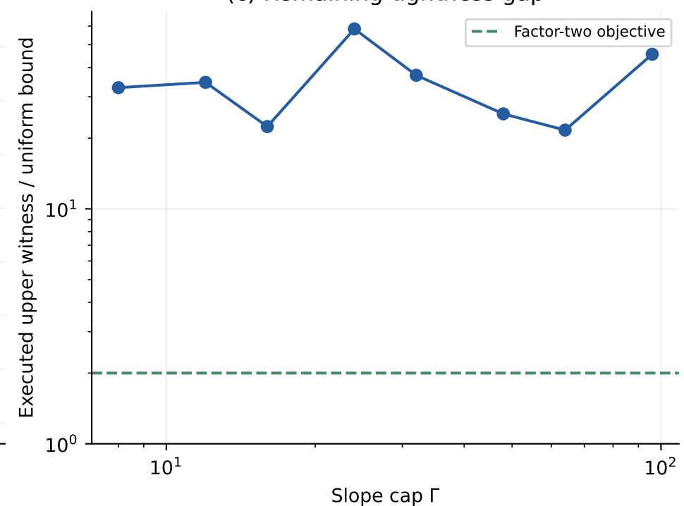
(c) Remaining tightness gap
