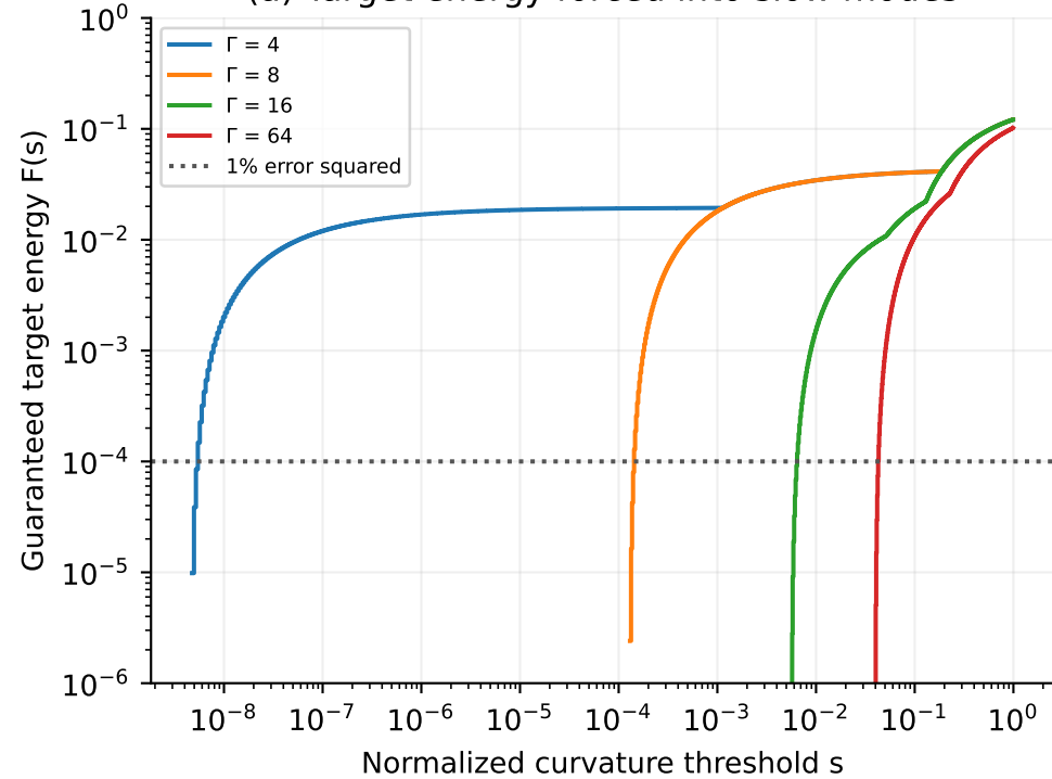
(a) Target energy forced into slow modes
