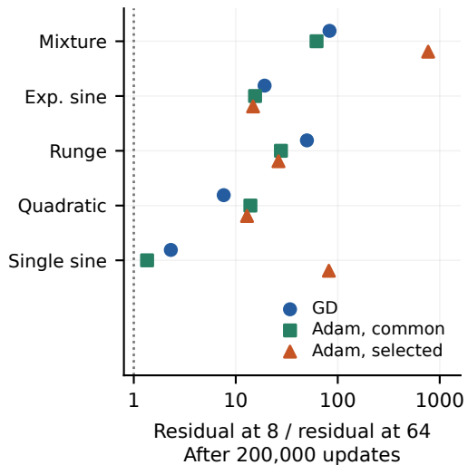
C GD and Adam: five targets
