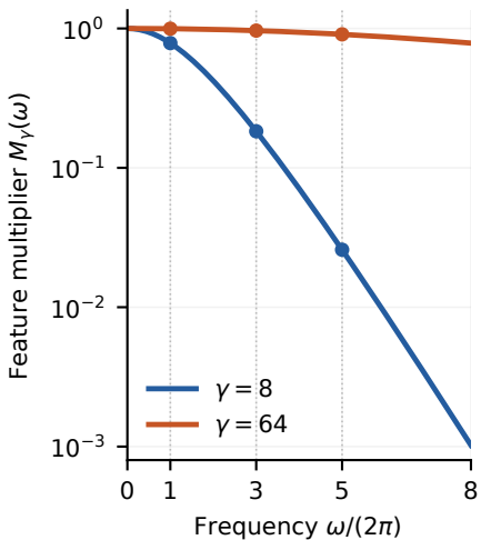
A Gamma filters fine scales
