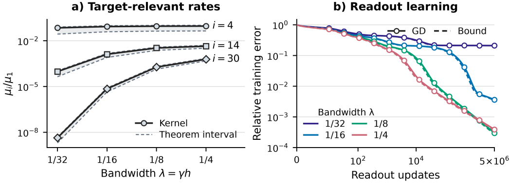
Figure 3: Small slopes weaken kernel directions and delay readout learning. Width W = 512 ; target f(x) = [\sin(2\pi x) + \frac{1}{2}\sin(6\pi x) + \frac{1}{4}\sin(14\pi x)]/\sqrt{21/32} on [-1, 1] . (a) Kernel ratios \mu_i/\mu_1 (outlined markers) and intervals from Theorem A.1 (dashed boundaries, shading) for three ranks carrying substantial target energy. Lines connect ordered ranks; eigenvectors change with bandwidth. (b) Executed frozen-readout GD errors (solid, hollow markers) and square roots of Theorem 3.2’s lower bounds (dashed). The error bound combines theorem-derived rate bounds with all resolved target projections onto the frozen kernel’s eigenvectors. Errors are relative training RMS through five million updates; geometry and protocol are in Appendix B.
