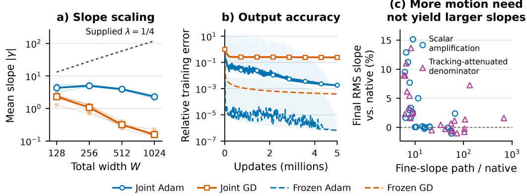
Figure 4: Joint training leaves a scale and accuracy gap. Panels (a,b): mixed-sine target on [-1, 1] ; five million updates. Joint training uses five seeds and one recipe per width and optimizer, selected by median final validation error. (a) Mean absolute slope versus total width, including halos. Faint curves show seed means; outlined markers show pooled means. (b) At W = 512 , relative training RMS error for joint training (solid) and frozen readouts on the supplied \lambda = 1/4 dictionary (dashed). Joint curves show seed medians after binning. Shading preserves temporal extrema and, for joint training, seed spread. (c) Adam intervention responses over 10k updates from a shared 130k checkpoint. Each point compares an intervention with its matched native control: accumulated fine-slope path versus percentage difference in final RMS slope. The 48 comparisons span six target families, widths 705 and 1409, and two seeds; they are separate from the experiments in (a,b). Greater motion can increase acquisition but need not produce a substantially larger endpoint scale. All altered pulse-end RMS bandwidths remain below 0.013, compared with the construction reference 0.25. The dotted line in (a) marks that supplied construction scale, not a universal acquisition threshold. Protocol and target for (a,b) are in Appendix D.
