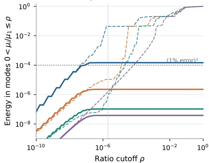
B Adam leaves slow-mode residual
