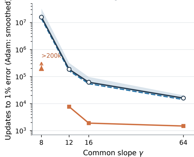
C Error lower bound forces delay
