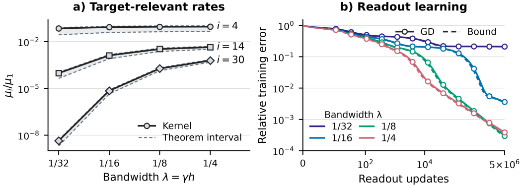
Figure 3: Small slopes weaken kernel directions and delay readout learning. Width W = 512 ; target f(x) = [\sin(2\pi x) + \frac{1}{2}\sin(6\pi x) + \frac{1}{4}\sin(14\pi x)]/\sqrt{21/32} on [-1, 1] . (a) Kernel ratios \mu_i/\mu_1 (outlined markers) and intervals from Theorem A.1 (dashed boundaries, shading) for three ranks carrying substantial target energy. Lines connect ordered ranks; eigenvectors change with bandwidth. (b) Executed frozen-readout GD errors (solid, hollow markers) and square roots of Theorem 3.2’s lower bounds (dashed). The error bound combines theorem-derived rate bounds with all resolved target projections onto the frozen kernel’s eigenvectors. Errors are relative training RMS through five million updates; geometry and protocol are in Appendix B.
