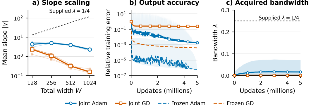
Figure 4: Joint training leaves a scale and accuracy gap. Mixed-sine target on [-1, 1] ; five million updates. Joint training uses five seeds and one recipe per width and optimizer, selected by median final validation error. (a) Mean absolute slope versus total width, including halos. Faint curves show seed means; outlined markers show pooled means. (b) At W = 512 , relative training RMS error for joint training (solid) and frozen readouts on the supplied \lambda = 1/4 dictionary (dashed). Joint curves show seed medians after binning. Shading preserves temporal extrema and, for joint training, seed spread. (c) Mean bandwidth \lambda = h_W |\gamma| for the same joint runs, with one population standard deviation across neurons and seeds, clipped at zero. Dotted lines in (a,c) mark the supplied construction scale, not a universal acquisition threshold. Protocol and target are in Appendix B.
