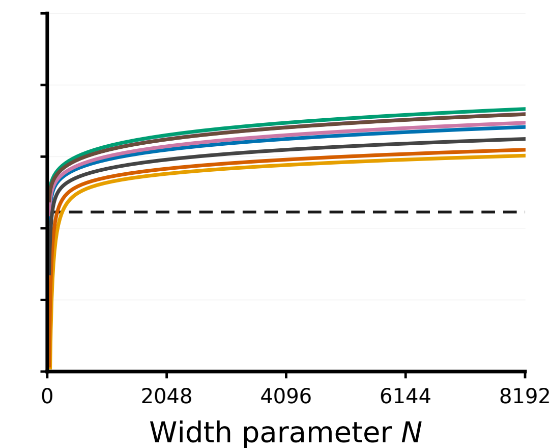
SiLU
