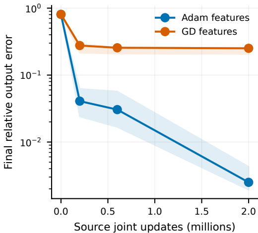
Frozen Adam readout restart
