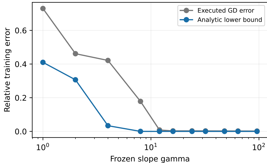
Sine mixture after 200k updates
