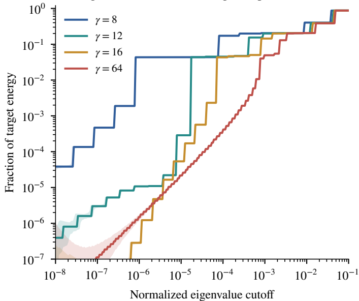
A Target-mass bounds and original spectrum
