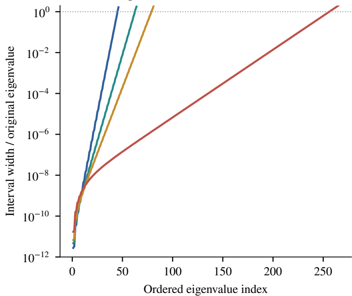
B Relative spectral enclosure width
