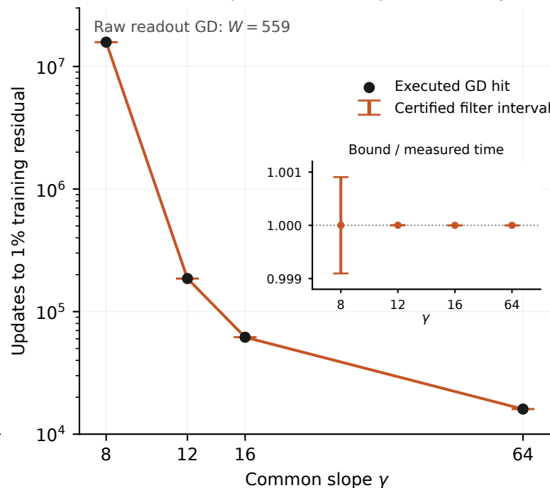
B Gamma predicts the acquisition delay
