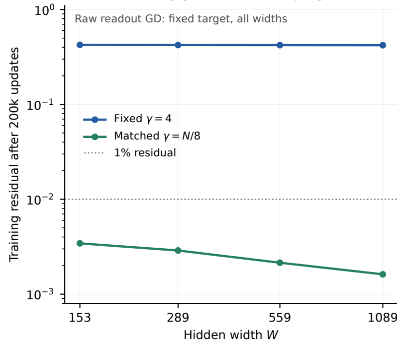
C Scaling gamma restores progress
