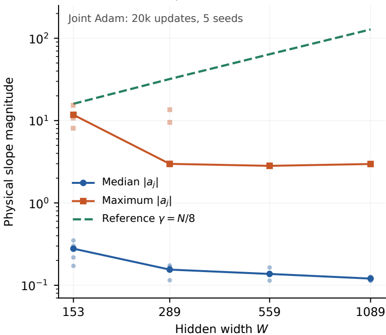
A Learned slopes miss the reference scale
