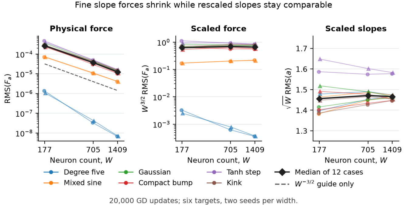
Figure 6: Wider populations have much weaker physical slope force at the 20k-update forks. Each width contains six targets and two seeds; points retain individual cases and larger markers summarize medians. The physical-force panel shows the decline in RMS effective fine slope gradient. Multiplying by W^{3/2} gives medians 0.628, 0.695, and 0.661; rescaled slope RMS values are 1.456, 1.471, and 1.466. Actual widths 177, 705, and 1409 correspond to reference resolutions 128, 512, and 1024. Force values use the retained modal audit. A power-law guide is a comparison, not a fitted asymptotic theorem.
