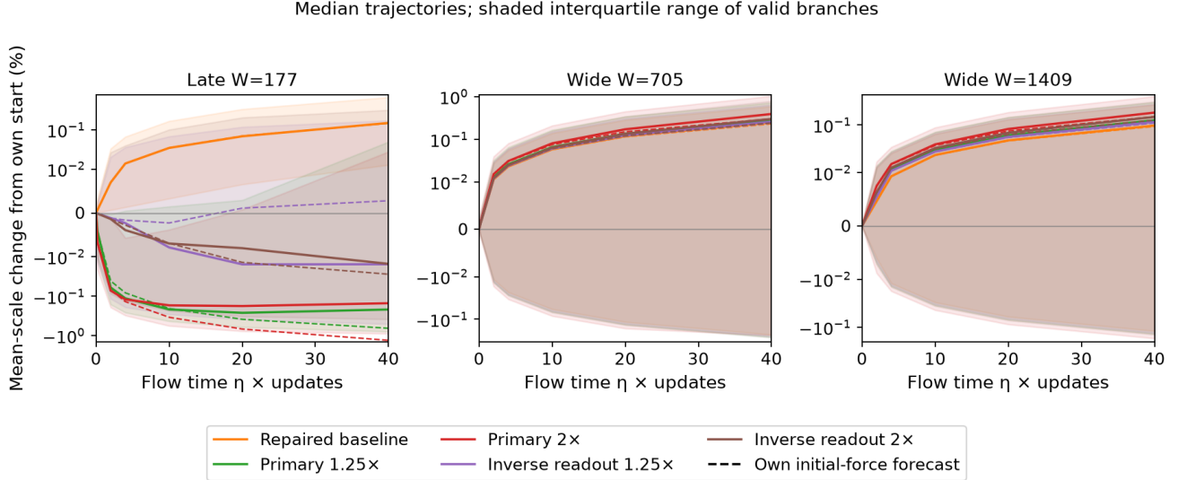
Figure 5: Finite geometry dilations followed by ordinary GD. Each curve starts after the imposed increase, so injected scale is excluded from learned motion. Solid curves are medians and shading is the interquartile range; dashed curves freeze each state’s own initial effective slope gradient. Left: 23 targets and two seeds, width 177, after 600k prior updates. Middle and right: six targets and two seeds per width, after 20k prior updates. Every branch continues for 20k updates at learning rate 0.002; flow time 40 means 20k updates. All six branches per checkpoint passed preparation and completed training. Primary and inverse identify readout repair references, not different GD rules. Different checkpoint ages prevent treating the three panels as a controlled width comparison.
