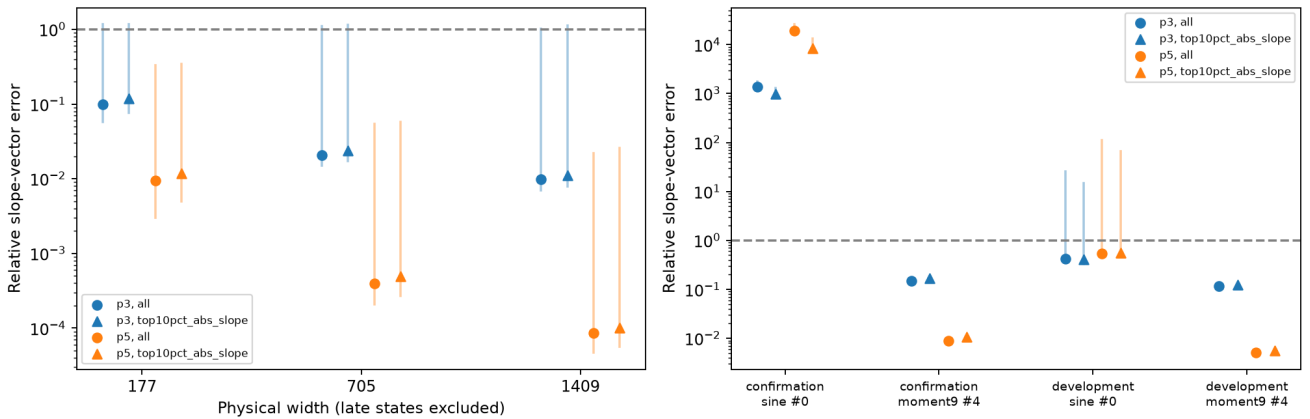
Figure 7: Quintic force accuracy is strong in the wide panel but fails in late sine. Each point is a median and each segment a full range. Left: 96 sampled states per width, comprising twelve cases and eight horizons. Right: four late cases kept separate; source indices in the labels are archive indices, not seeds. Blue is cubic, orange quintic; triangles restrict to the largest 10% of slopes. These are force reconstructions at actual states, not forecasts.
