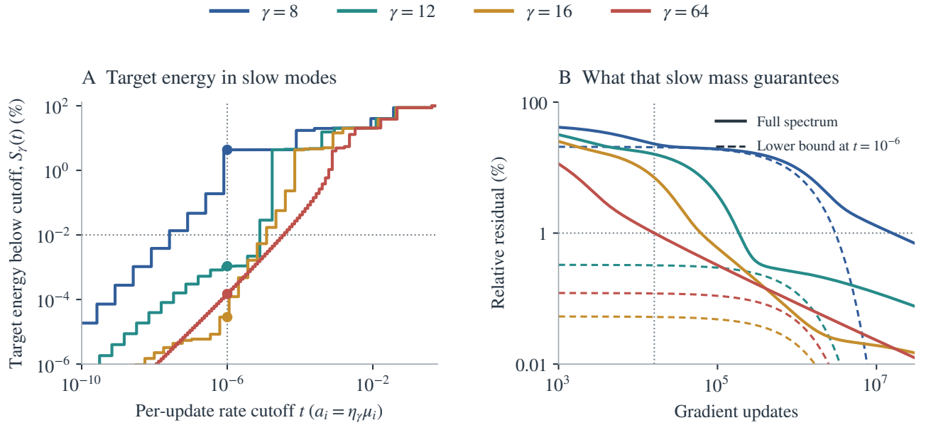
Figure 1: The missing link is target energy in slow modes. A shows S_\gamma(t) from the gamma-filtered finite kernels; dots mark t = 10^{-6} . The horizontal guide is target energy 10^{-4} , or 0.01%, corresponding to a 1% residual. B compares the full-spectrum residual predictions with the lower bounds \sqrt{S_\gamma(10^{-6})(1 - 10^{-6})^n} ; its horizontal guide is a 1% residual and its vertical guide is 16,013 updates. All curves here are calculations from the archived kernels, not executed trajectories. The spectra and cutoff bounds are FP64 diagnostics, not independently interval-certified spectral masses.
