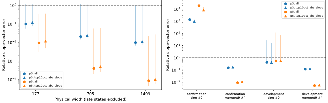
Figure 3: Quintic force accuracy is strong in the wide panel but fails in late sine. Each point is a median and each segment a full range. Left: 96 sampled states per width, comprising twelve cases and eight horizons. Right: four late cases kept separate; source indices in the labels are archive indices, not seeds. Blue is cubic, orange quintic; triangles restrict to the largest 10% of slopes. These are force reconstructions at actual states, not forecasts.
