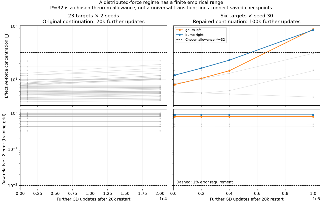
Figure 13: Test the structural assumption together with output error. Left: 23 targets and two seeds, original GD at width 705, starting after 20k updates and continued for 20k more. Right: six targets at seed 30, repaired baseline at the same width and restart age, continued for 100k updates. Top: force concentration, with the illustrative allowance 32. Bottom: raw relative training error, with the 1% criterion. The two highlighted longer runs leave the allowance while retaining large error. Lines connect retained checkpoints; they do not certify concentration between checkpoints. The separately recorded every-update error counters exclude a 1% crossing in these two longer continuations.
