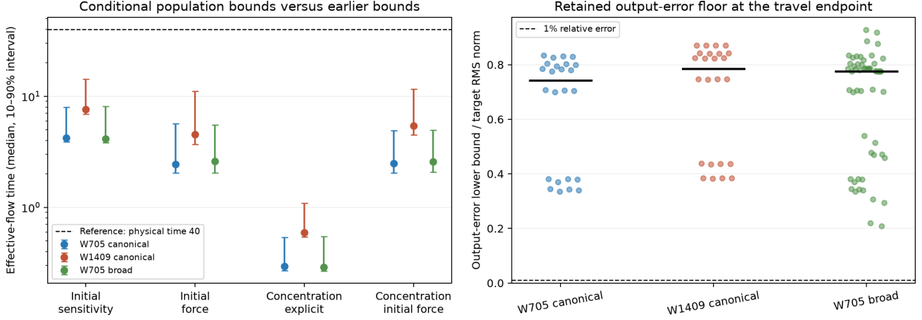
Figure 14: What the simpler assumption buys, and what remains unresolved. Left: median effective-flow duration and 10th–90th percentile range under four sufficient bounds. The concentration methods assume future I_F \leq 32 ; the other two use initial data only. The dashed reference is physical time 40, not a certified GD conversion. Right: output-error floors at the concentration/initial-force bound’s endpoint. The original six-target groups have four seeds each; the broad width-705 group has 58 states across 23 targets and includes the original group. All starts have age 20k. These are FP64 evaluations of sufficient inequalities, not interval certificates or independent target samples.
