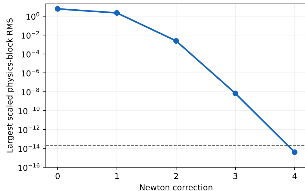
Solve starts from zero coefficients
