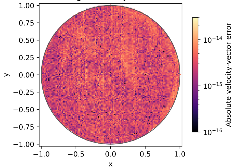
Error against analytical check
