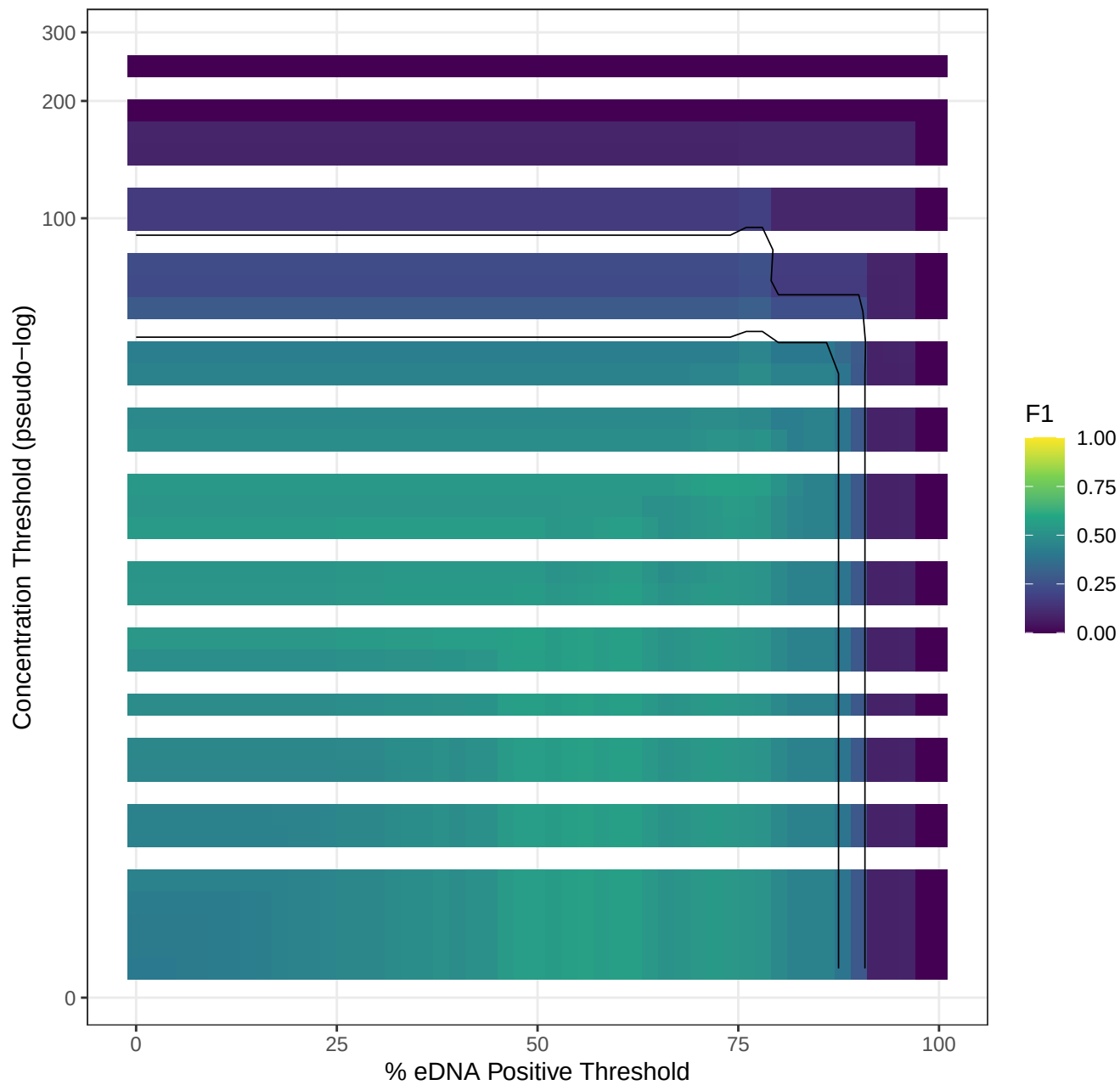
2D Boolean Search: AND Rule F1 (CPUE = 0.040)
