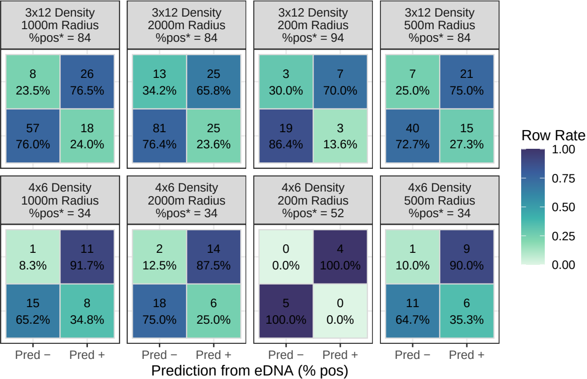
Site-Level Confusion Matrices across Radial Buffers and Sampling Regimes (
