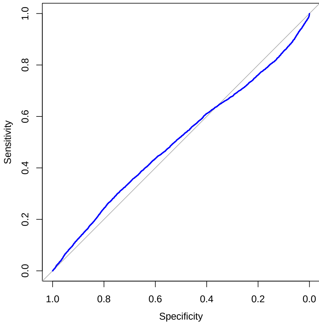
ROC Curve (2025)
